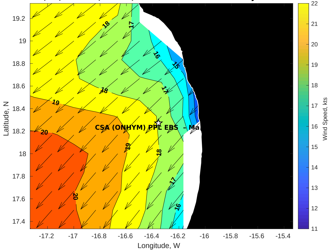
GFS Winds (kts) for CSA (ONHYM) PPL EBS - Mauritania at 10-Jan-2026 09:00:00
