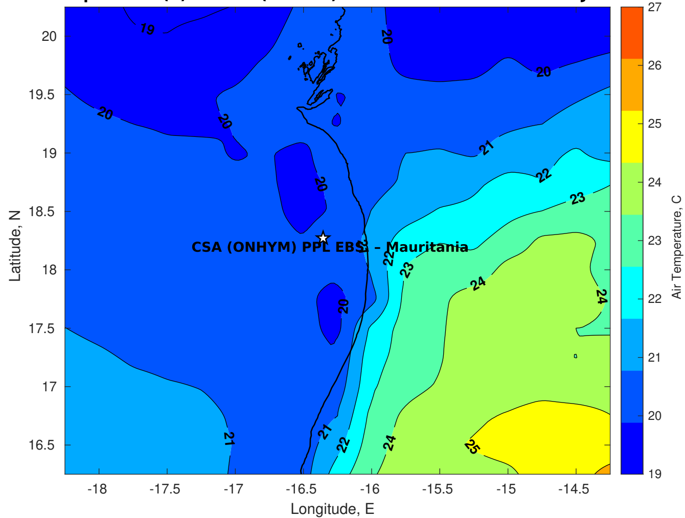
Air Temperature (C) for CSA (ONHYM) PPL EBS - Mauritania at 10-Jan-2026
