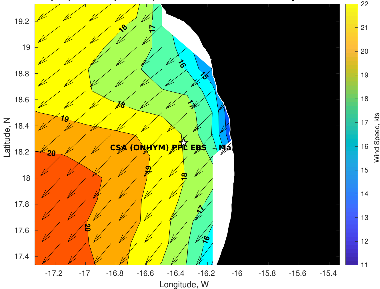
GFS Winds (kts) for CSA (ONHYM) PPL EBS - Mauritania at 10-Jan-2026 09:00:00
