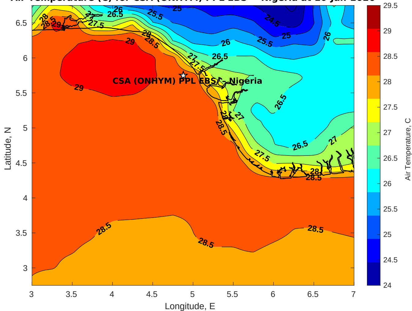
Air Temperature (C) for CSA (ONHYM) PPL EBS - Nigeria at 10-Jan-2026
