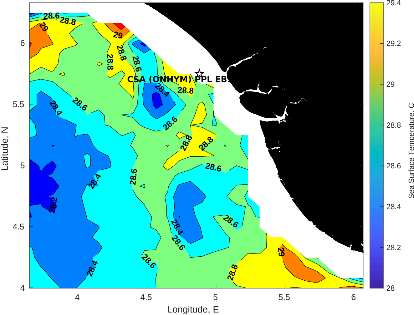
SST for CSA (ONHYM) PPL EBS - Nigeria at 09-Jan-2026 00:00:00
