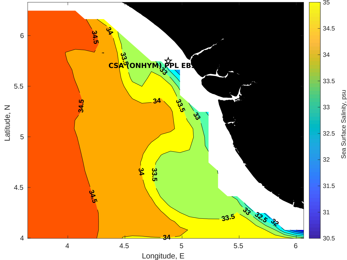
Surface Salinity for CSA (ONHYM) PPL EBS - Nigeria at 09-Jan-2026 00:00:00
