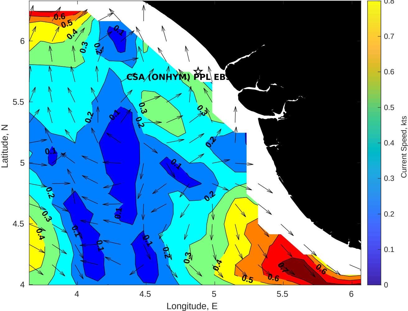
Surface Currents for CSA (ONHYM) PPL EBS - Nigeria at 09-Jan-2026 00:00:00
