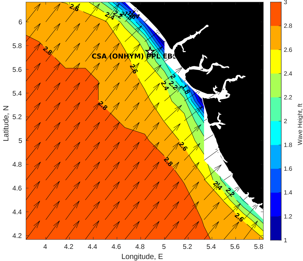
GFS Wave Height (ft) for CSA (ONHYM) PPL EBS - Nigeria at 10-Jan-2026 09:00:00
