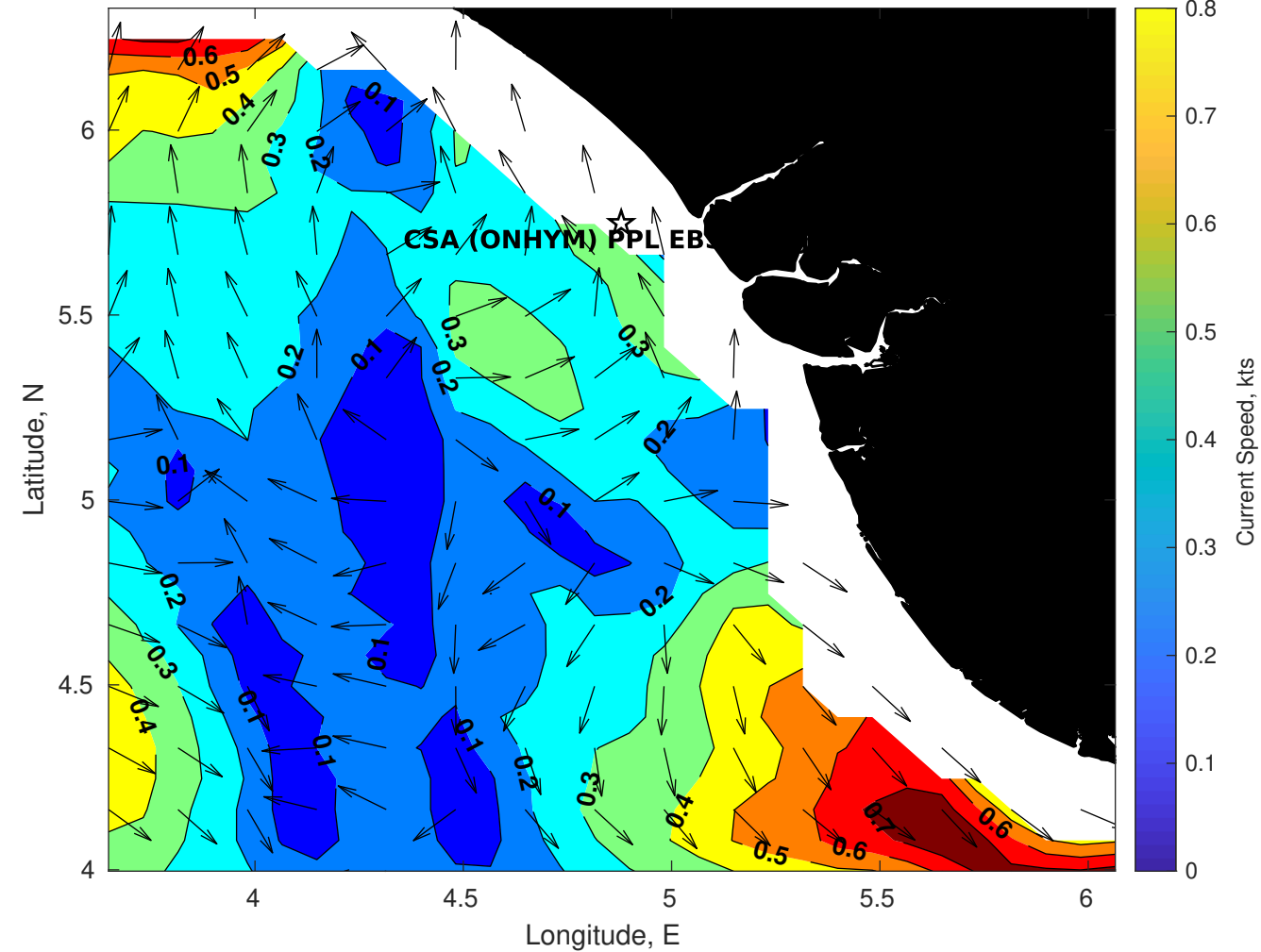
Surface Currents for CSA (ONHYM) PPL EBS - Nigeria at 09-Jan-2026 00:00:00
