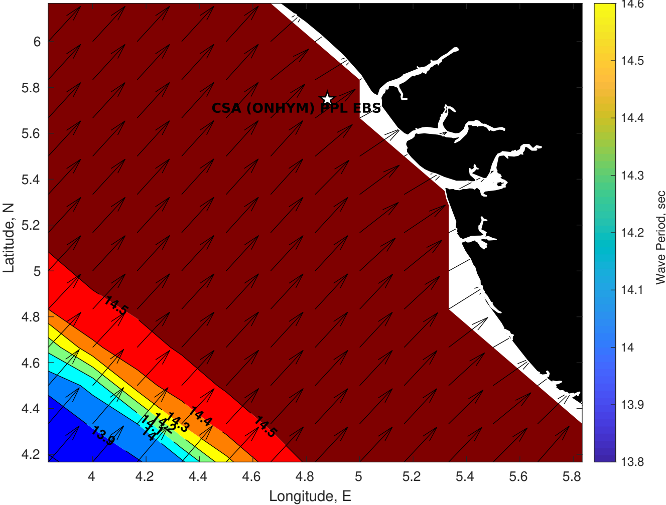
GFS Wave Period (sec) for CSA (ONHYM) PPL EBS - Nigeria at 10-Jan-2026 09:00:00
