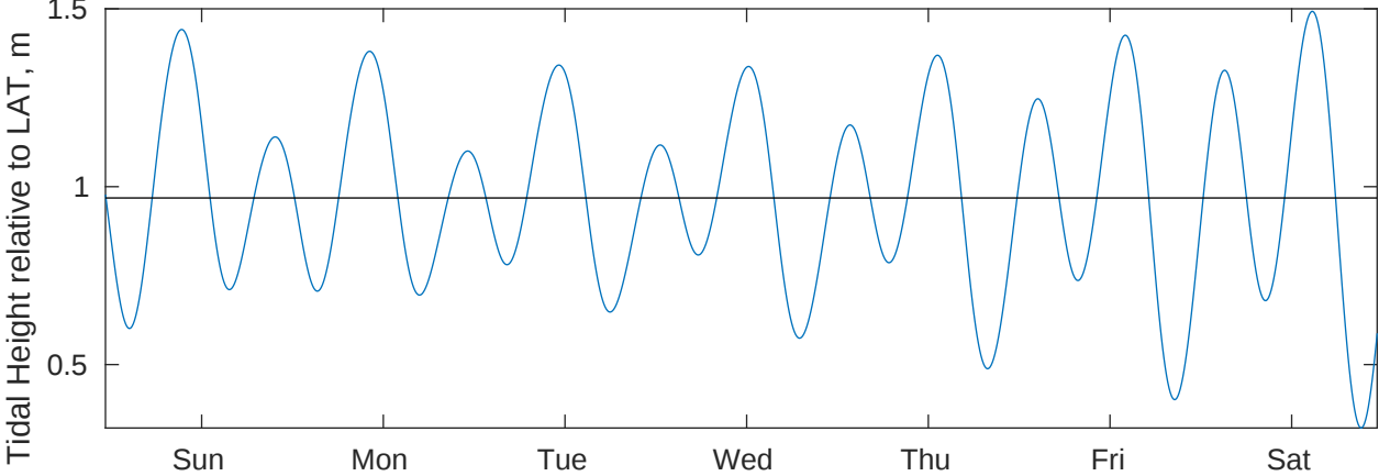
Tidal Currents and Heights for CSA (ONHYM) PPL EBS - Nigeria at 20260110
