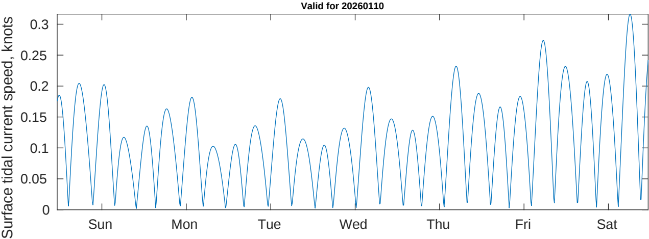
Tidal Currents and Heights for CSA (ONHYM) PPL EBS - Nigeria at 20260110
