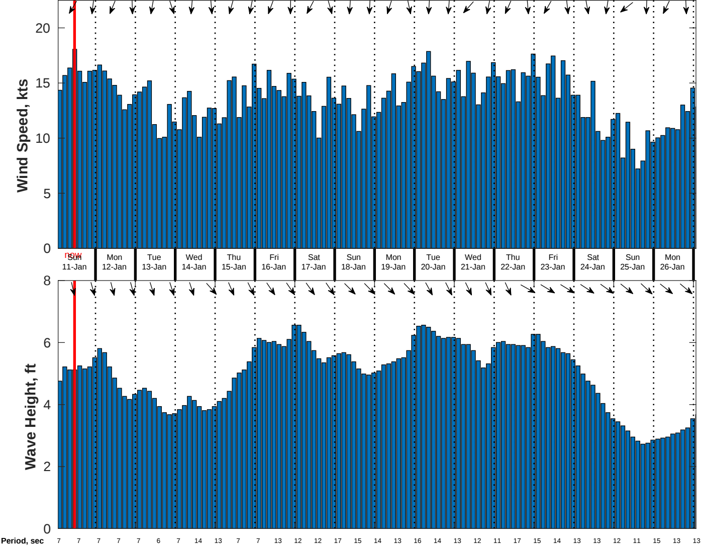
Wind & Wave Forecast for CSA (ONHYM) PPL EBS - Senegal from 10-Jan-2026 01:00:00 to 26-Jan-2026 01:00:00
