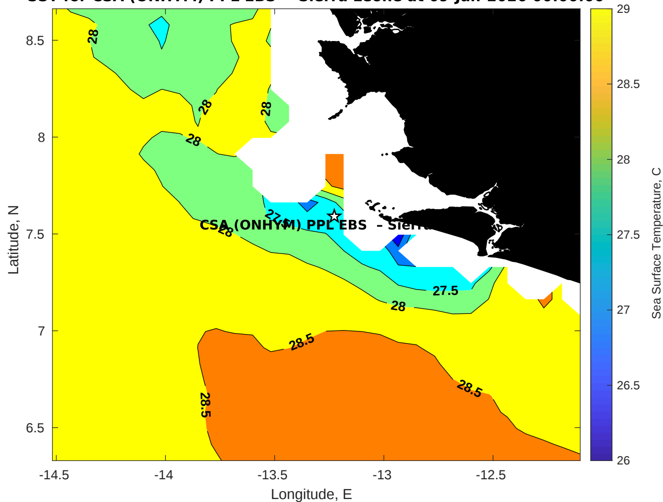
SST for CSA (ONHYM) PPL EBS - Sierra Leone at 09-Jan-2026 00:00:00
