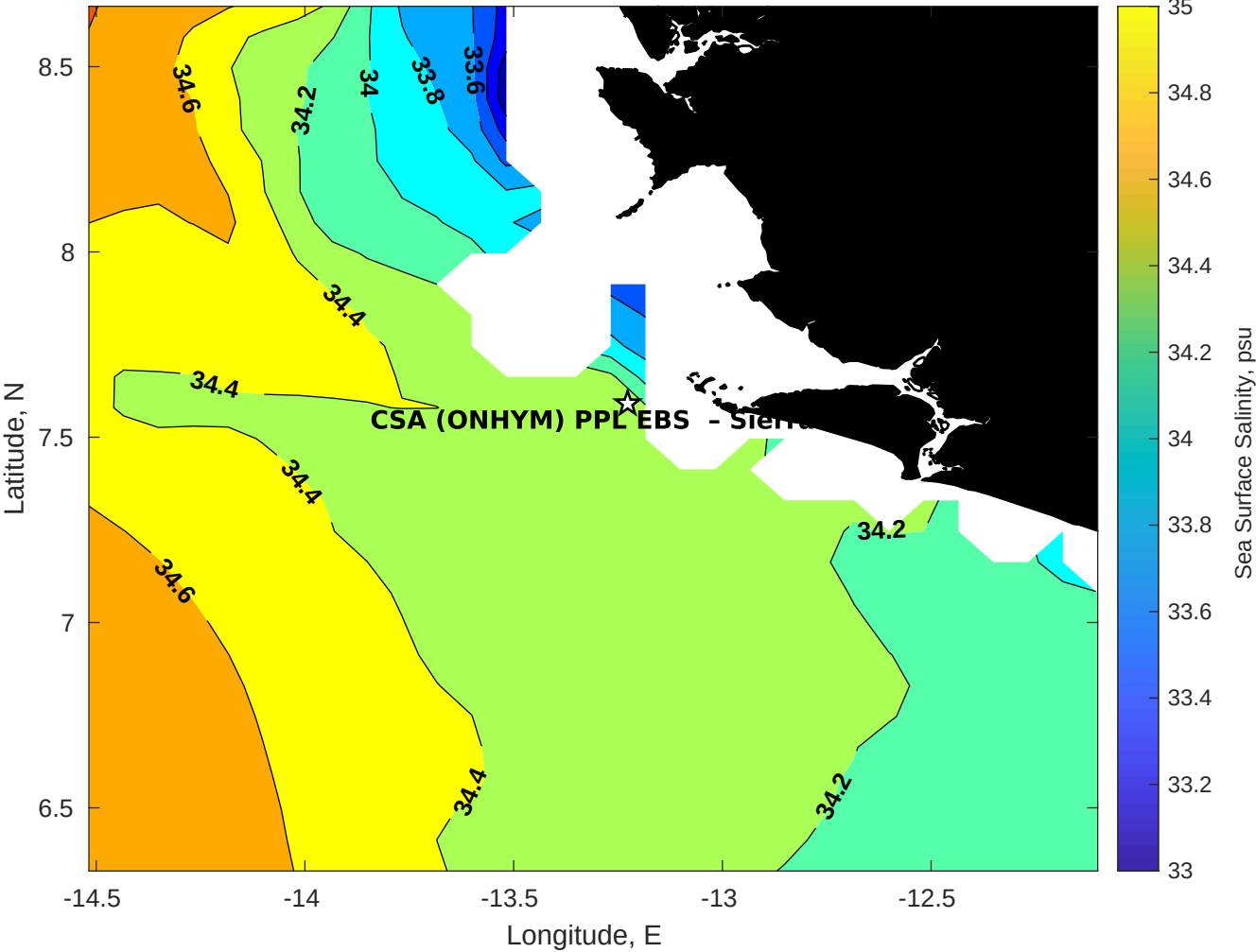
Surface Salinity for CSA (ONHYM) PPL EBS - Sierra Leone at 09-Jan-2026 00:00:00
