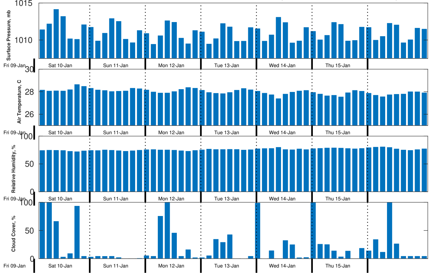
Met Forecast for CSA (ONHYM) PPL EBS - Sierra Leone from 10-Jan-2026 00:00:00 to 17-Jan-2026 00:00:00
