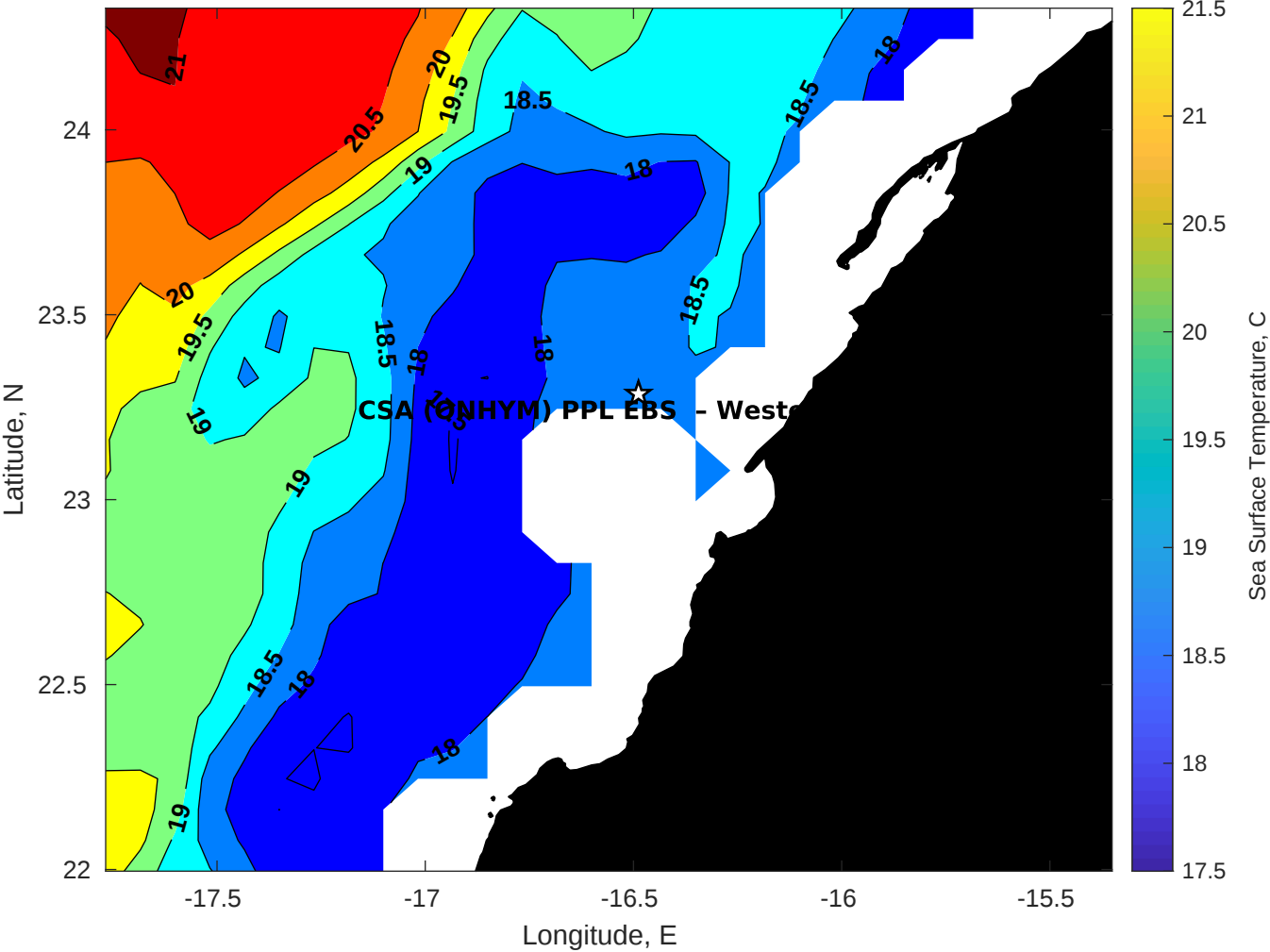
SST for CSA (ONHYM) PPL EBS - Western Sahara at 09-Jan-2026 00:00:00
