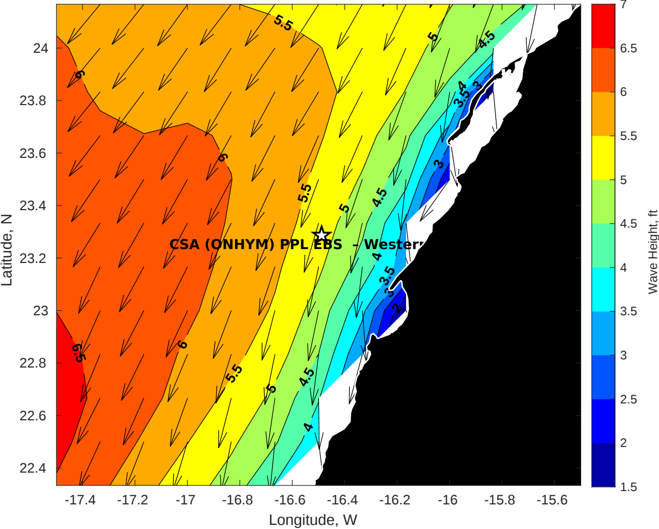
GFS Wave Height (ft) for CSA (ONHYM) PPL EBS - Western Sahara at 10-Jan-2026 09:00:00
