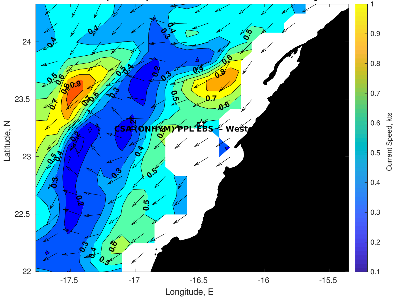
Surface Currents for CSA (ONHYM) PPL EBS - Western Sahara at 09-Jan-2026 00:00:00
