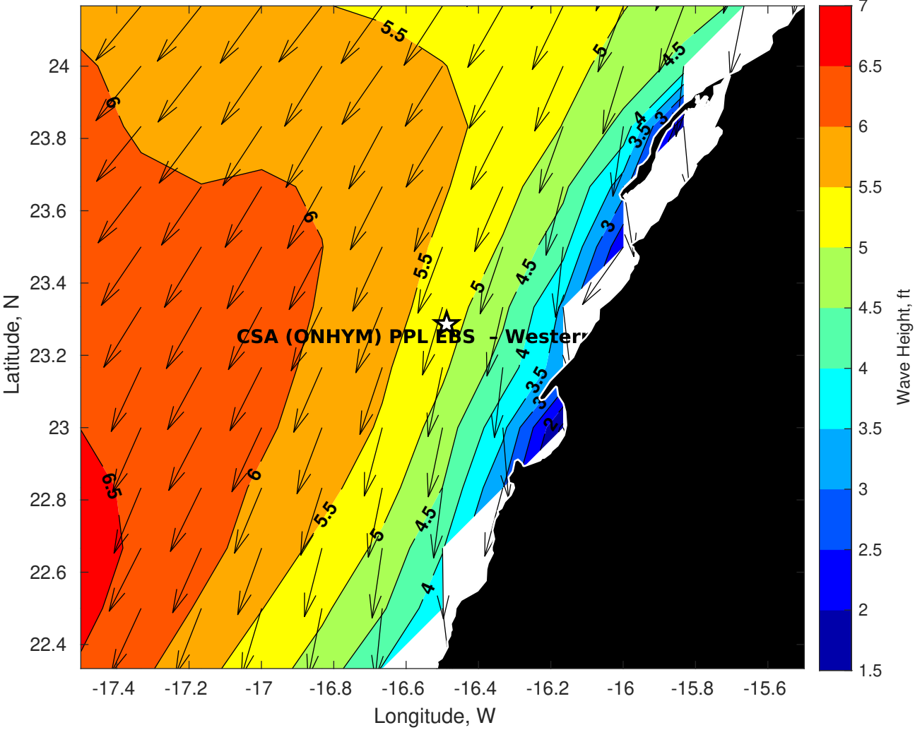
GFS Wave Height (ft) for CSA (ONHYM) PPL EBS - Western Sahara at 10-Jan-2026 09:00:00
