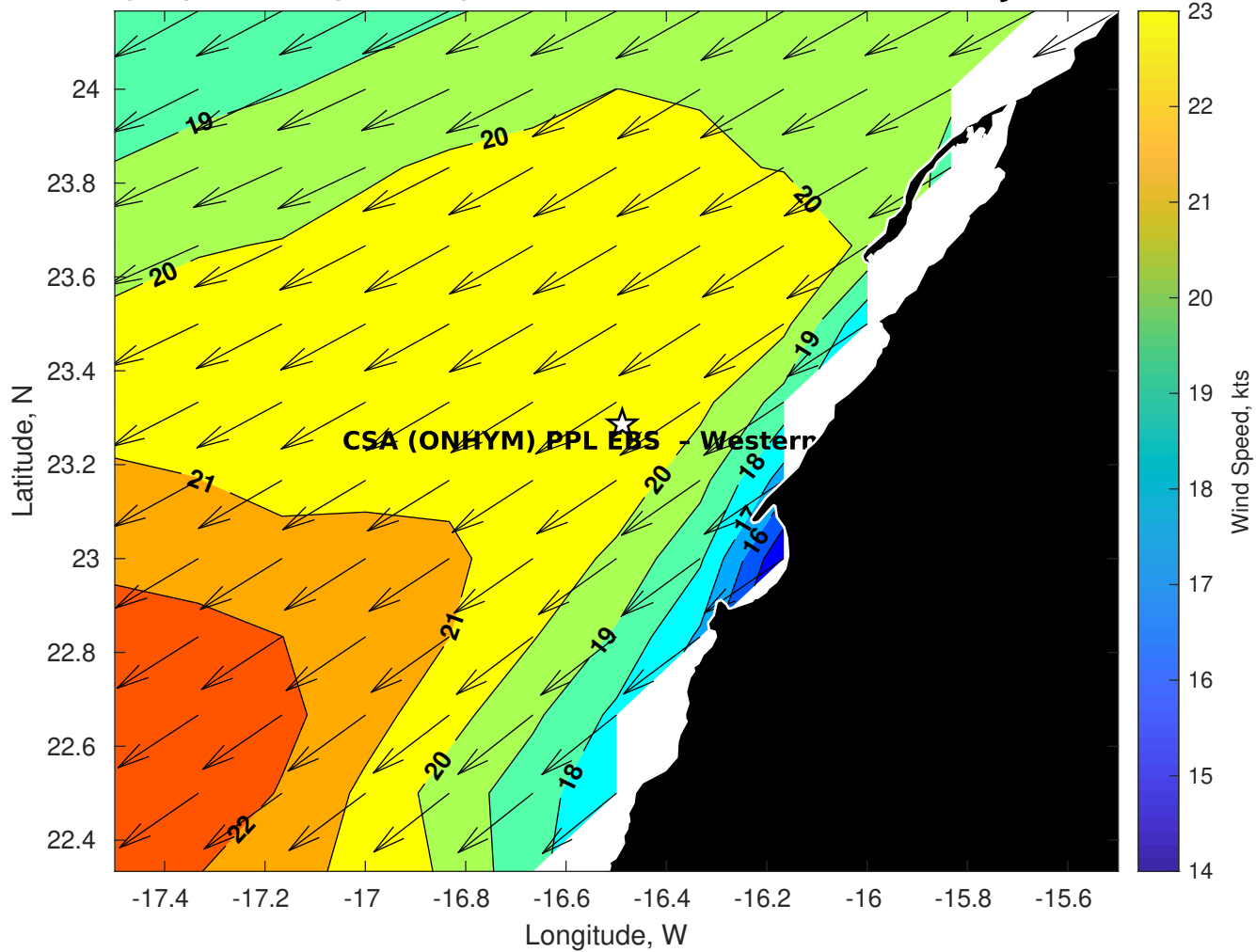
GFS Winds (kts) for CSA (ONHYM) PPL EBS - Western Sahara at 10-Jan-2026 09:00:00
