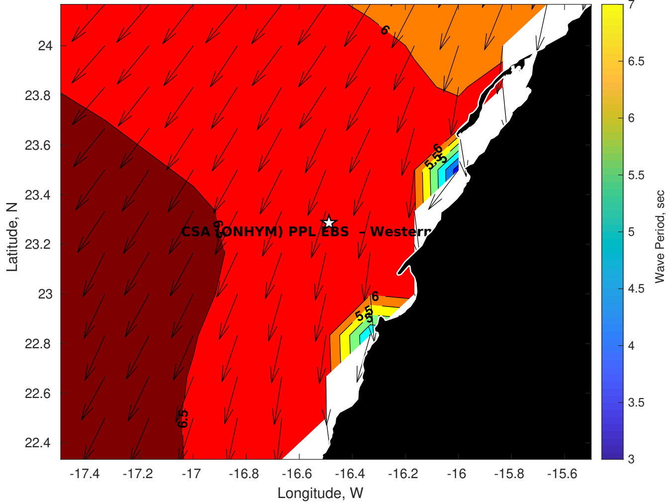
GFS Wave Period (sec) for CSA (ONHYM) PPL EBS - Western Sahara at 10-Jan-2026 09:00:00
