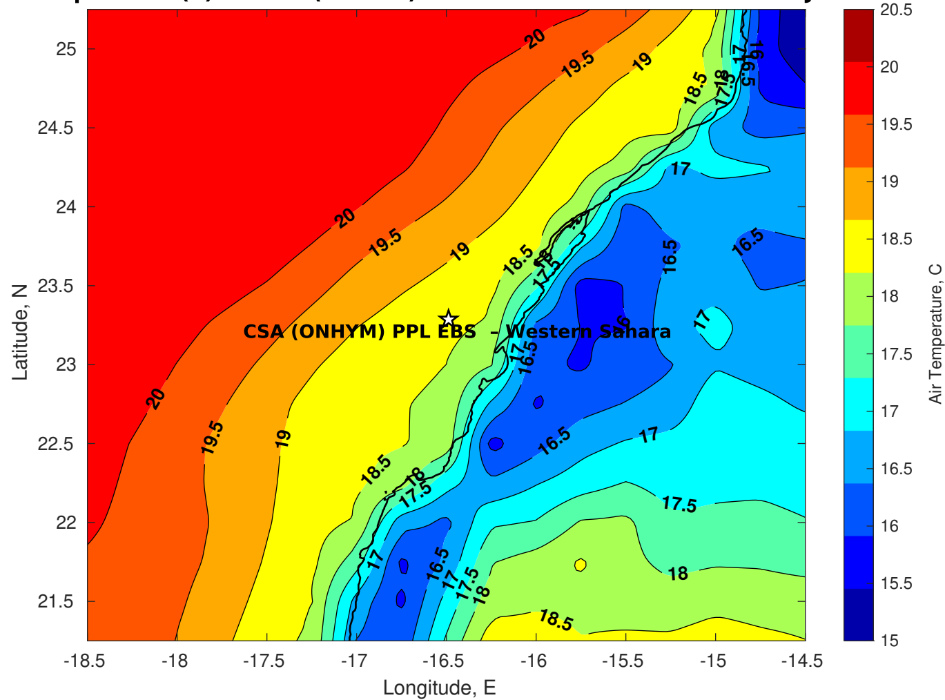
Air Temperature (C) for CSA (ONHYM) PPL EBS - Western Sahara at 10-Jan-2026
