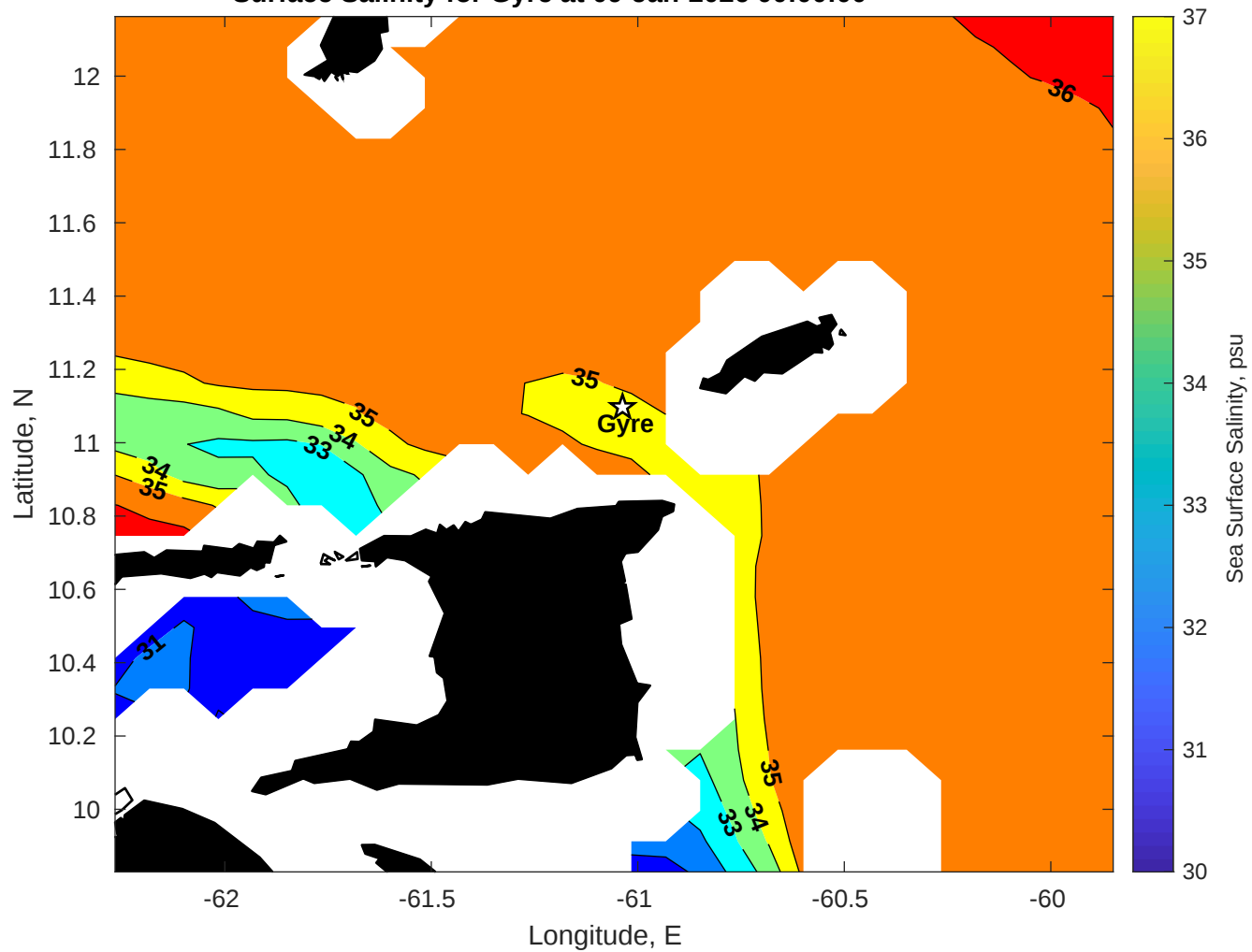
Surface Salinity for Gyre at 09-Jan-2026 00:00:00
