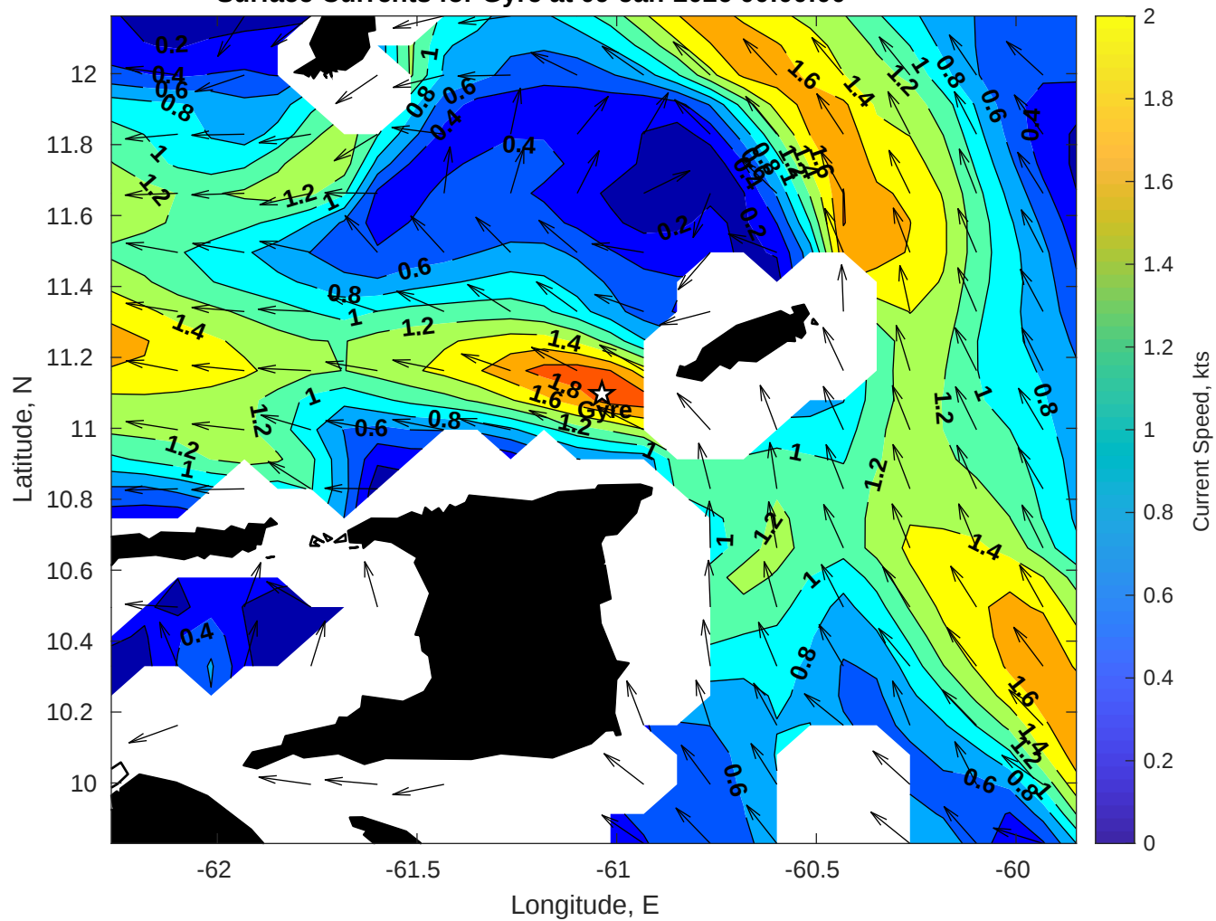
Surface Currents for Gyre at 09-Jan-2026 00:00:00
