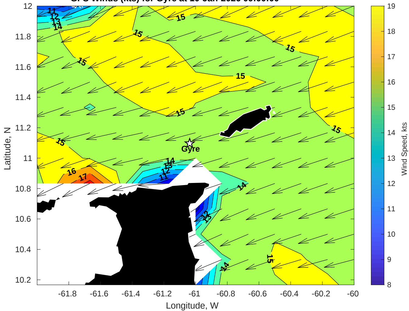
GFS Winds (kts) for Gyre at 10-Jan-2026 09:00:00
