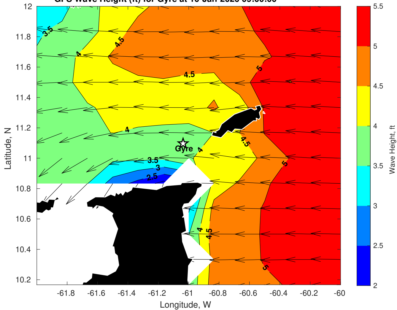
GFS Wave Height (ft) for Gyre at 10-Jan-2026 09:00:00
