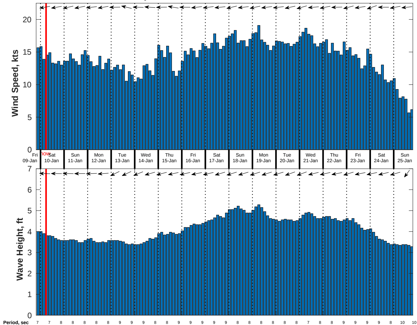
Wind & Wave Forecast for Gyre from 09-Jan-2026 20:00:00 to 25-Jan-2026 20:00:00
