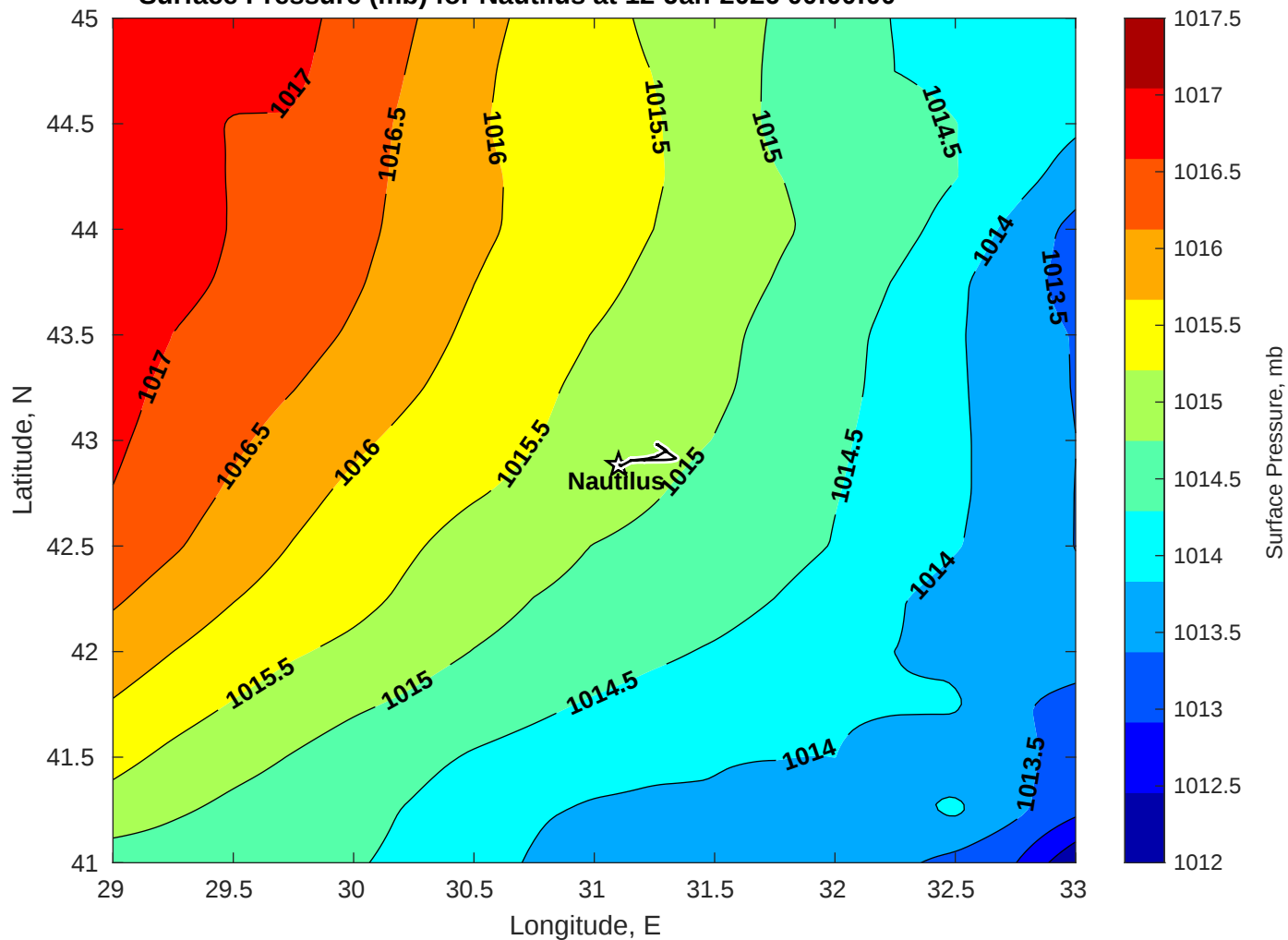
Surface Pressure (mb) for Nautilus at 12-Jan-2026 00:00:00
