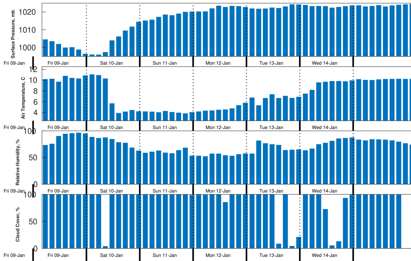
Met Forecast for Nautilus from 10-Jan-2026 00:00:00 to 17-Jan-2026 00:00:00
