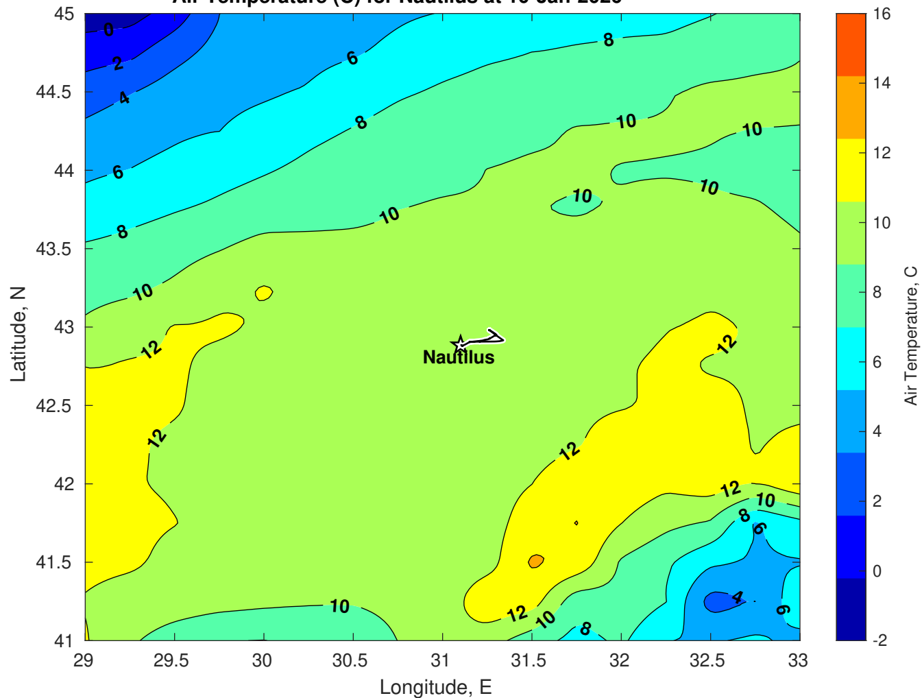
Air Temperature (C) for Nautilus at 10-Jan-2026
