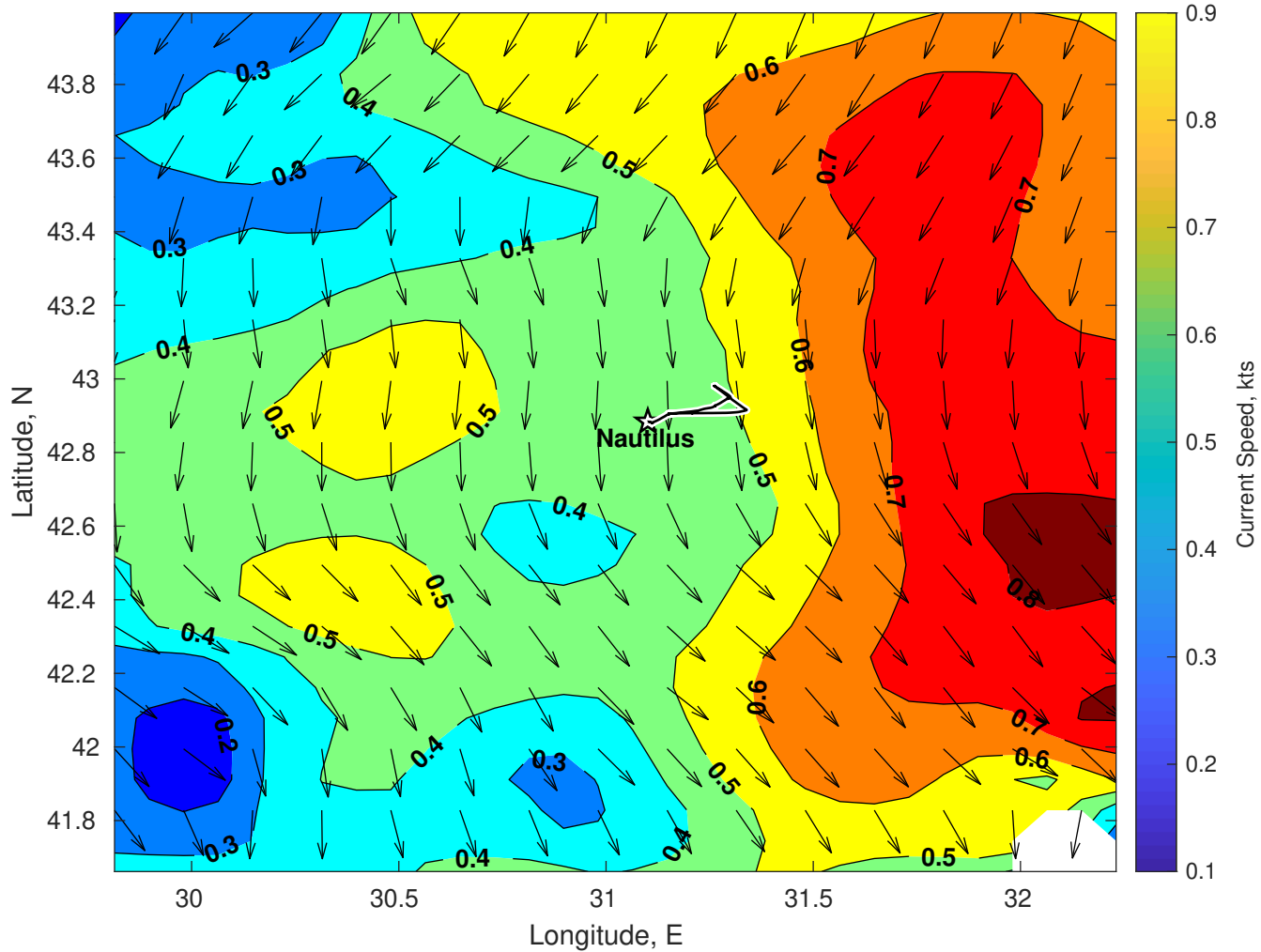
Surface Currents for Nautilus at 09-Jan-2026 00:00:00
