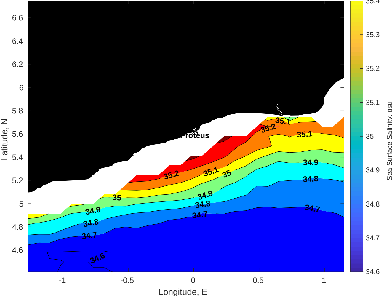
Surface Salinity for Proteus at 09-Jan-2026 00:00:00
