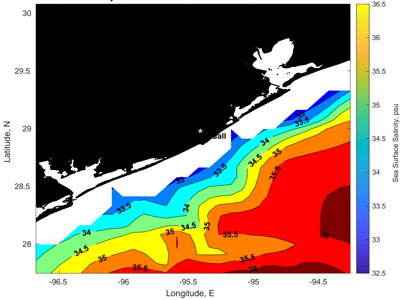
Surface Salinity for Brooks McCall at 10-Jan-2026 00:00:00
