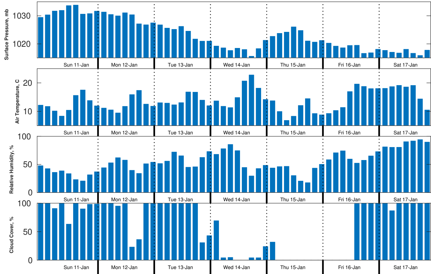
Met Forecast for Brooks McCall from 11-Jan-2026 00:00:00 to 18-Jan-2026 00:00:00
