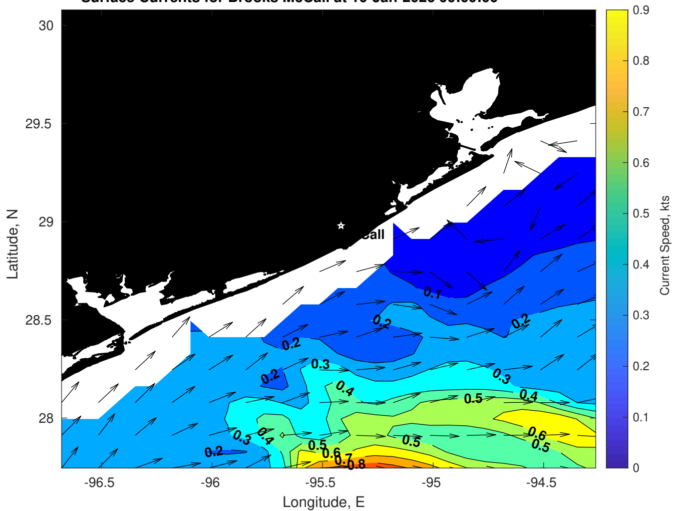
Surface Currents for Brooks McCall at 10-Jan-2026 00:00:00
