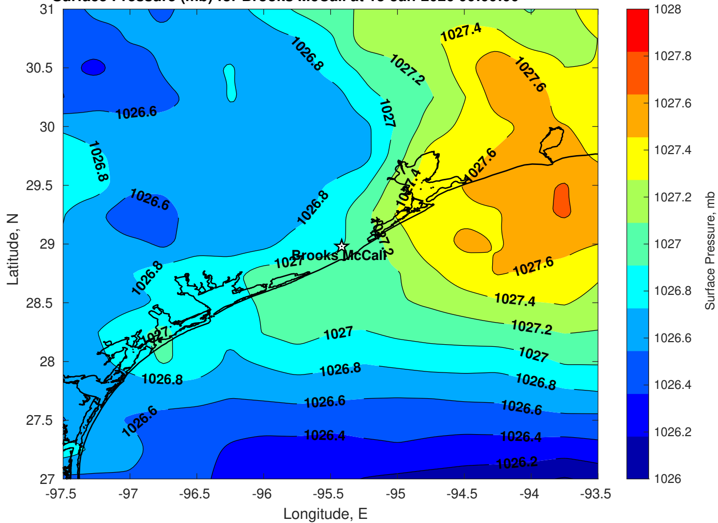
Surface Pressure (mb) for Brooks McCall at 13-Jan-2026 00:00:00
