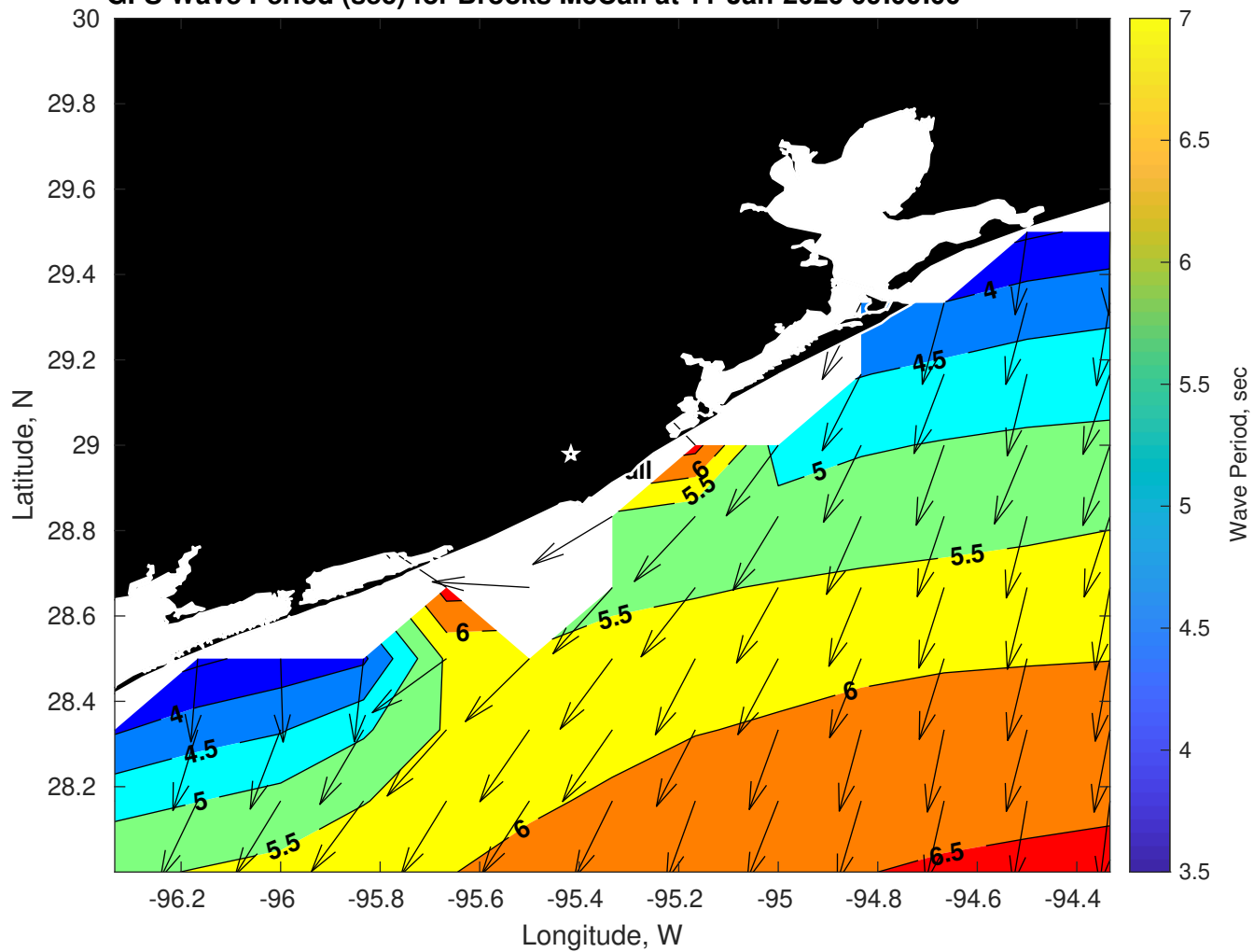
GFS Wave Period (sec) for Brooks McCall at 11-Jan-2026 09:00:00
