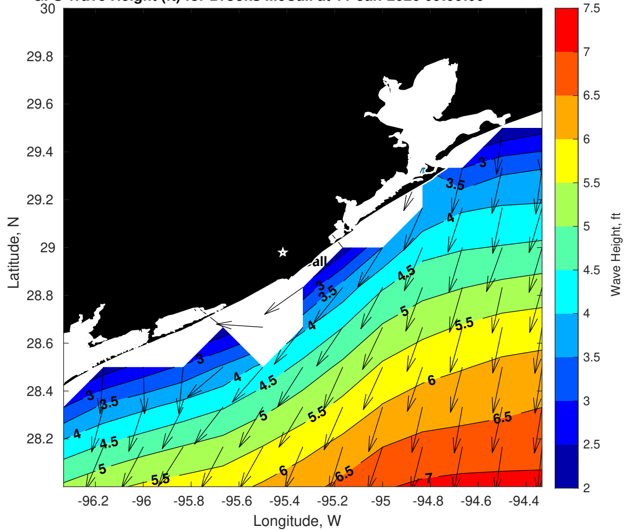
GFS Wave Height (ft) for Brooks McCall at 11-Jan-2026 09:00:00
