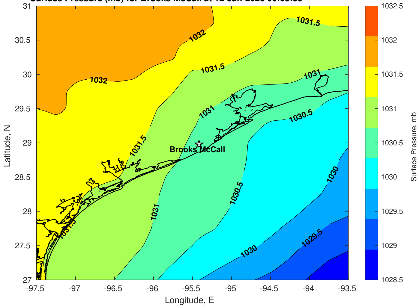
Surface Pressure (mb) for Brooks McCall at 12-Jan-2026 00:00:00
