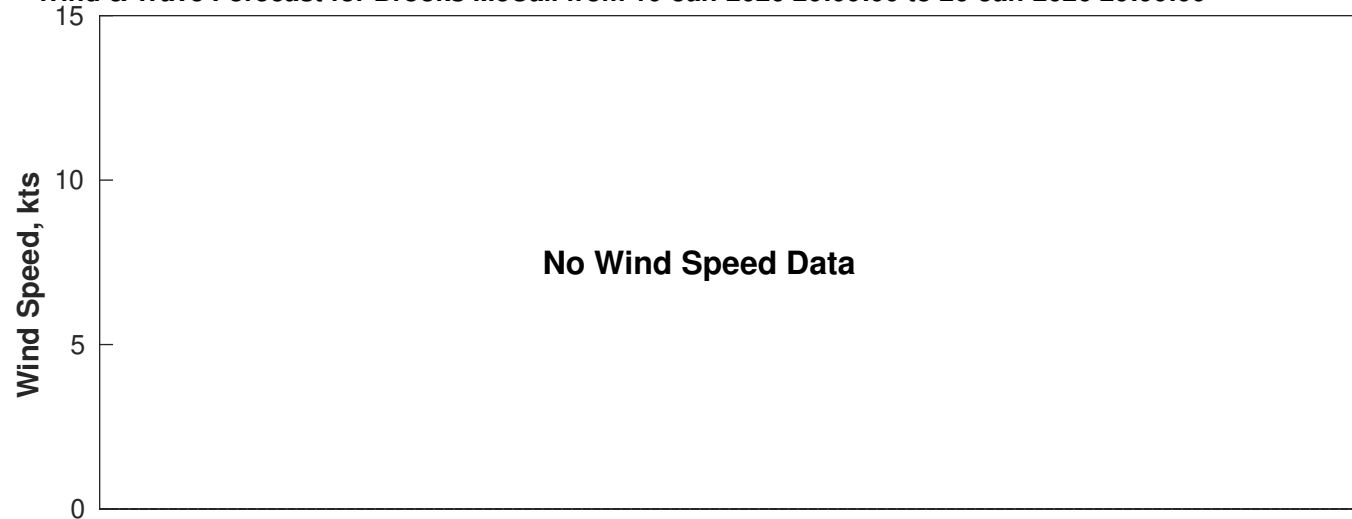
Wind & Wave Forecast for Brooks McCall from 10-Jan-2026 20:00:00 to 26-Jan-2026 20:00:00
