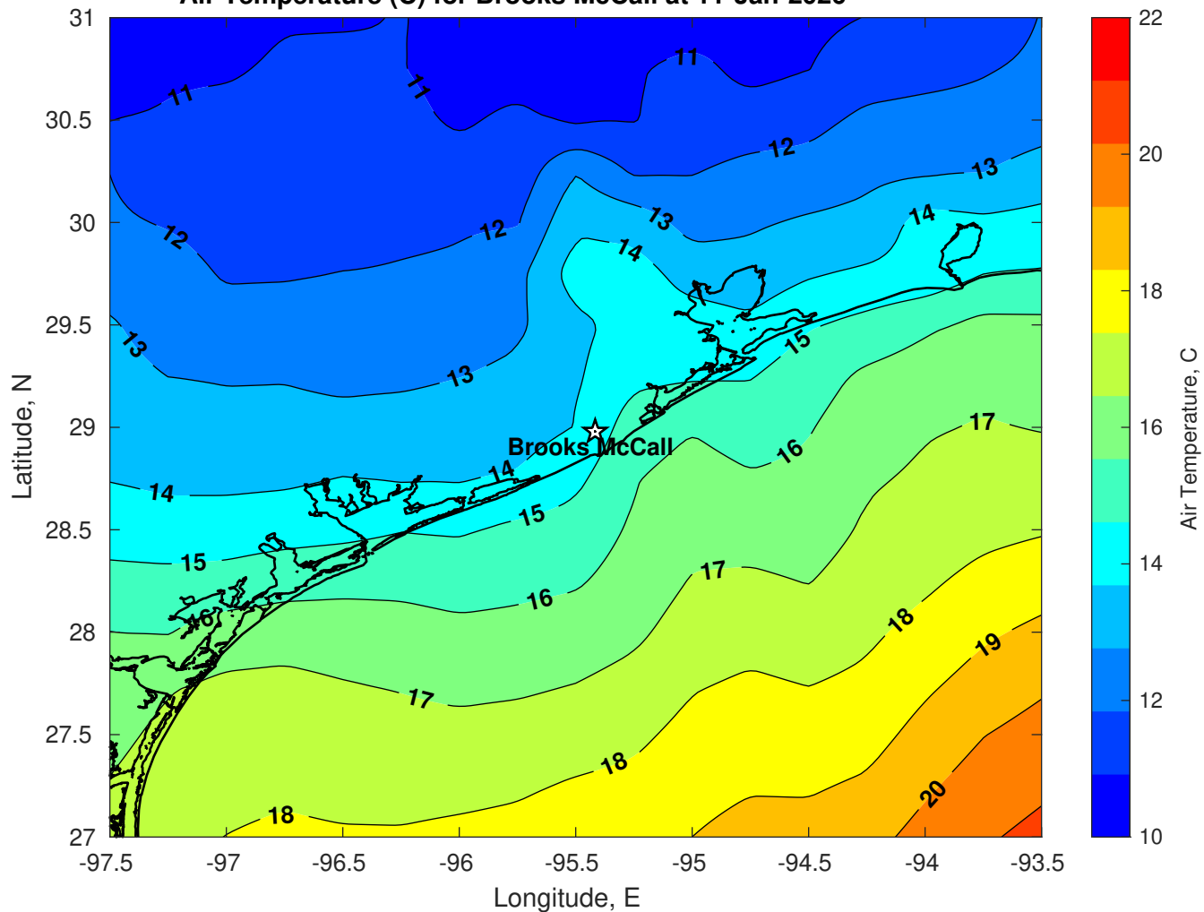
Air Temperature (C) for Brooks McCall at 11-Jan-2026
