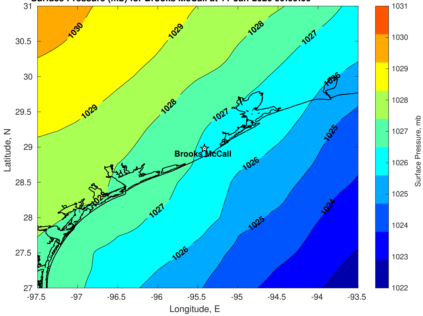
Surface Pressure (mb) for Brooks McCall at 11-Jan-2026 00:00:00
