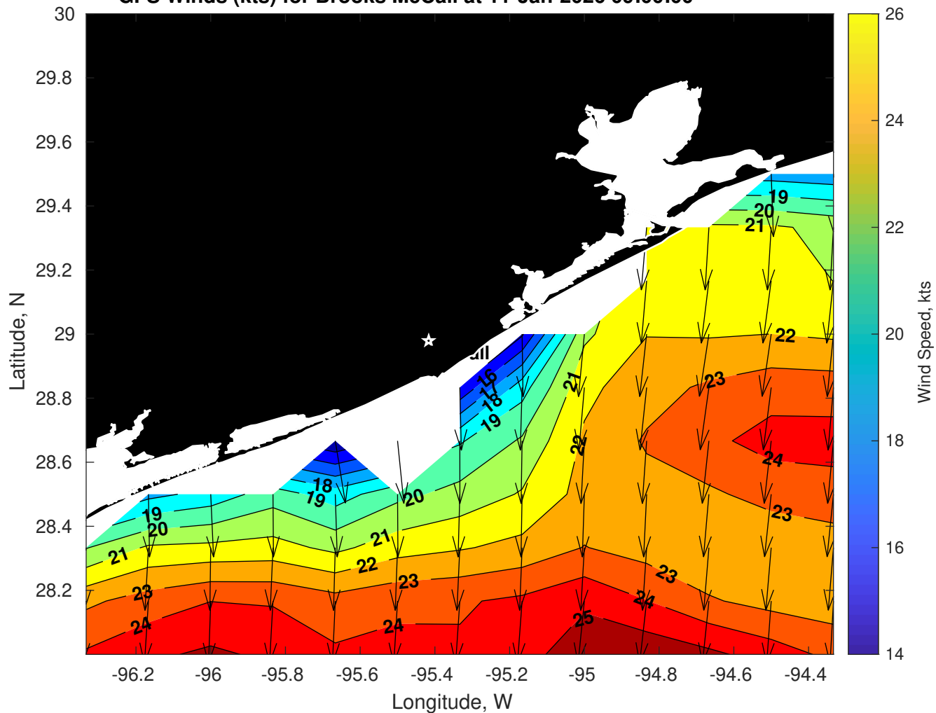
GFS Winds (kts) for Brooks McCall at 11-Jan-2026 09:00:00
