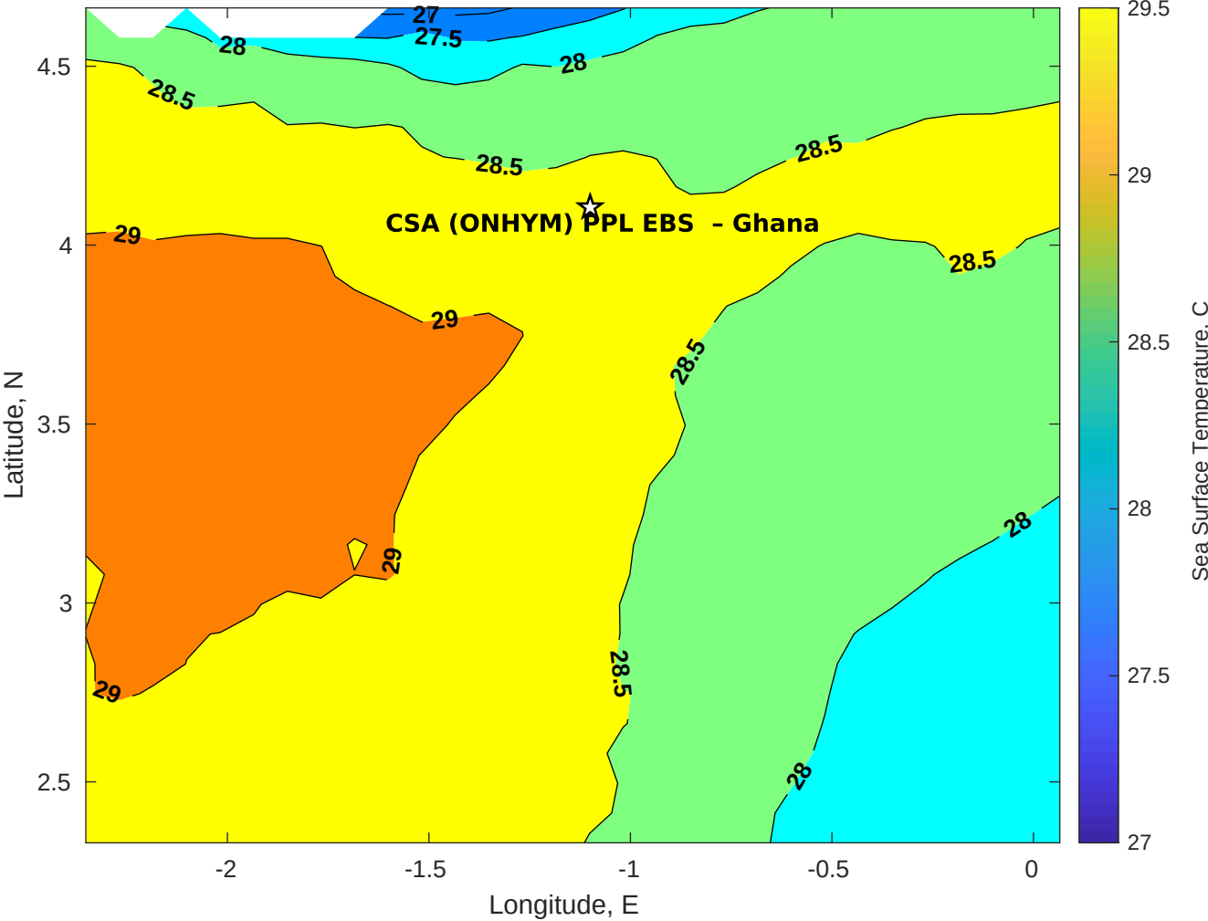
SST for CSA (ONHYM) PPL EBS - Ghana at 10-Jan-2026 00:00:00
