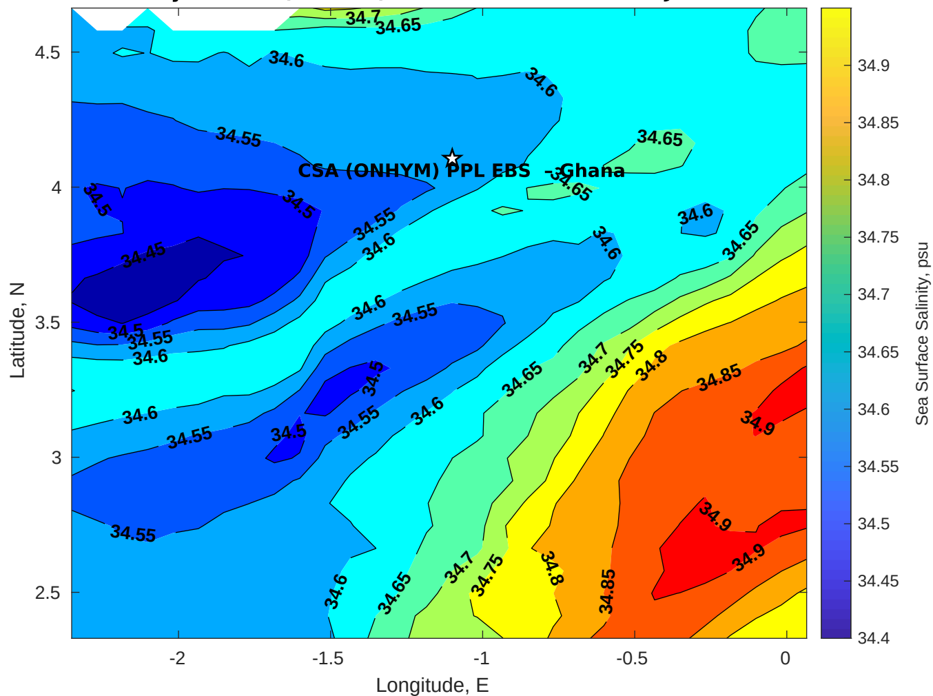
Surface Salinity for CSA (ONHYM) PPL EBS - Ghana at 10-Jan-2026 00:00:00
