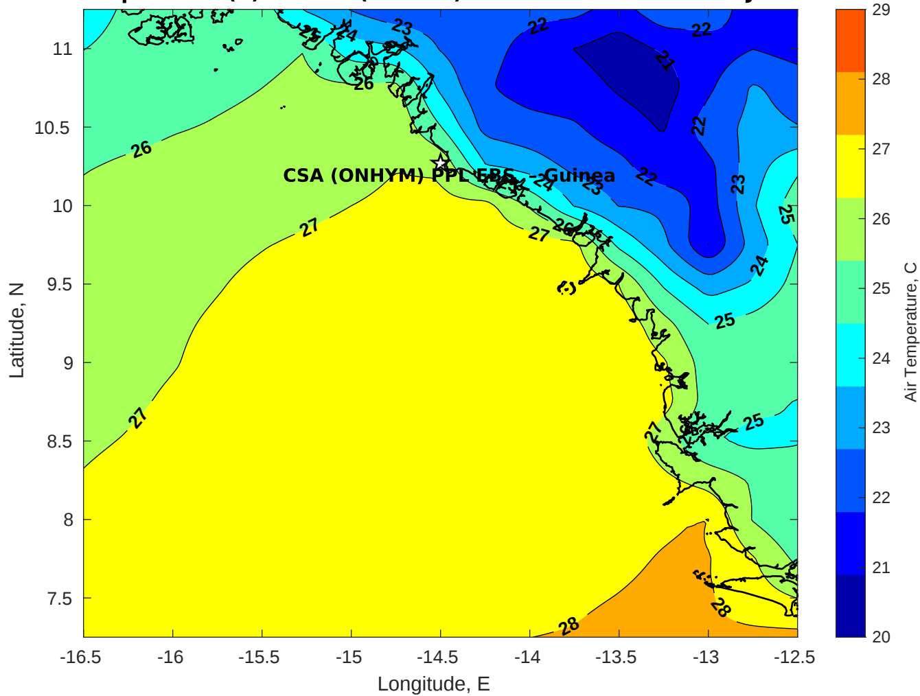
Air Temperature (C) for CSA (ONHYM) PPL EBS - Guinea at 11-Jan-2026
