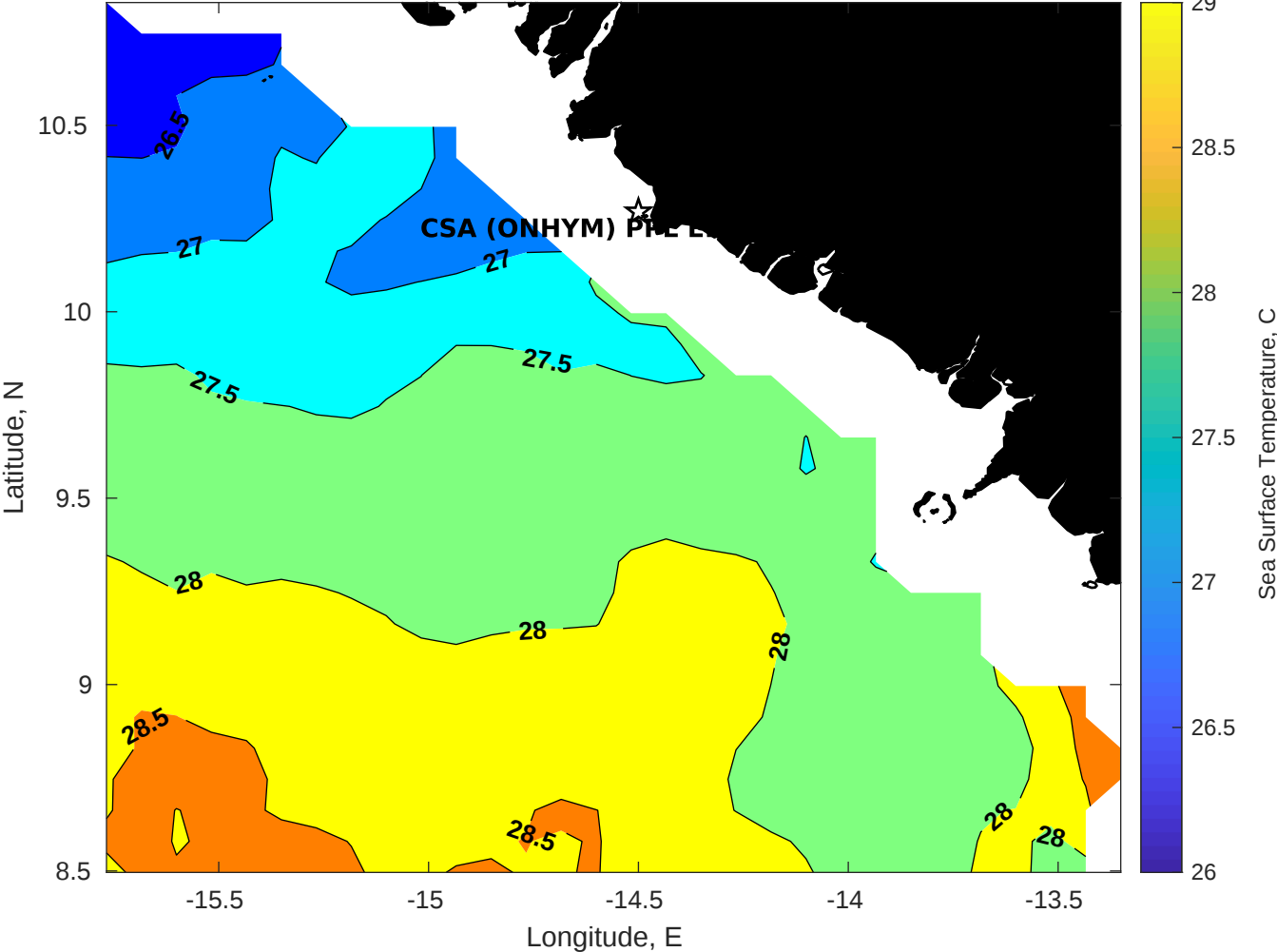
SST for CSA (ONHYM) PPL EBS - Guinea at 10-Jan-2026 00:00:00
