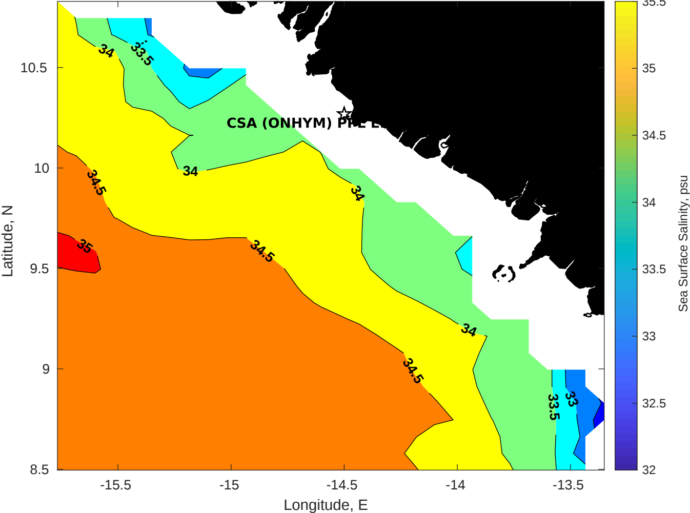
Surface Salinity for CSA (ONHYM) PPL EBS - Guinea at 10-Jan-2026 00:00:00
