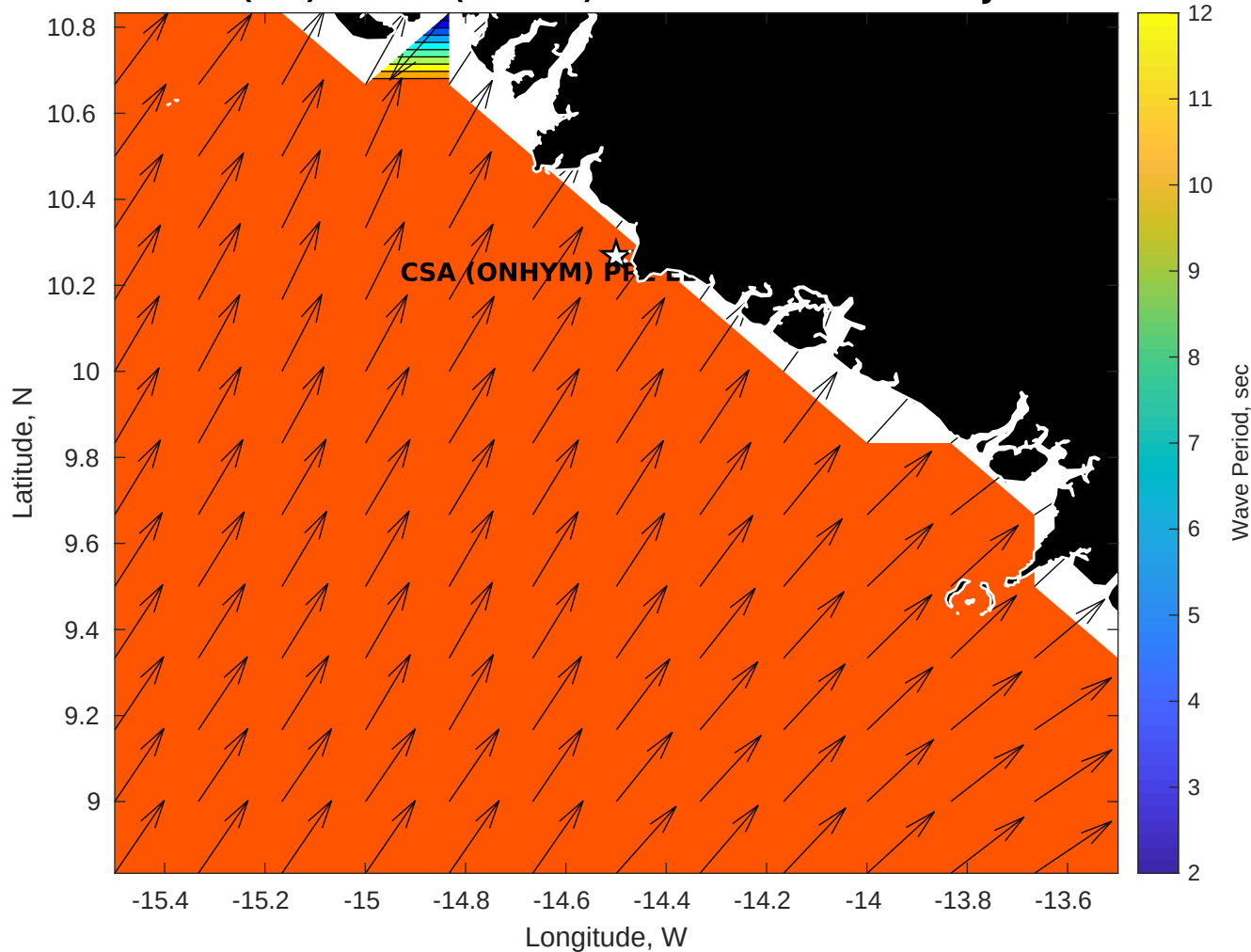
GFS Wave Period (sec) for CSA (ONHYM) PPL EBS - Guinea at 11-Jan-2026 09:00:00
