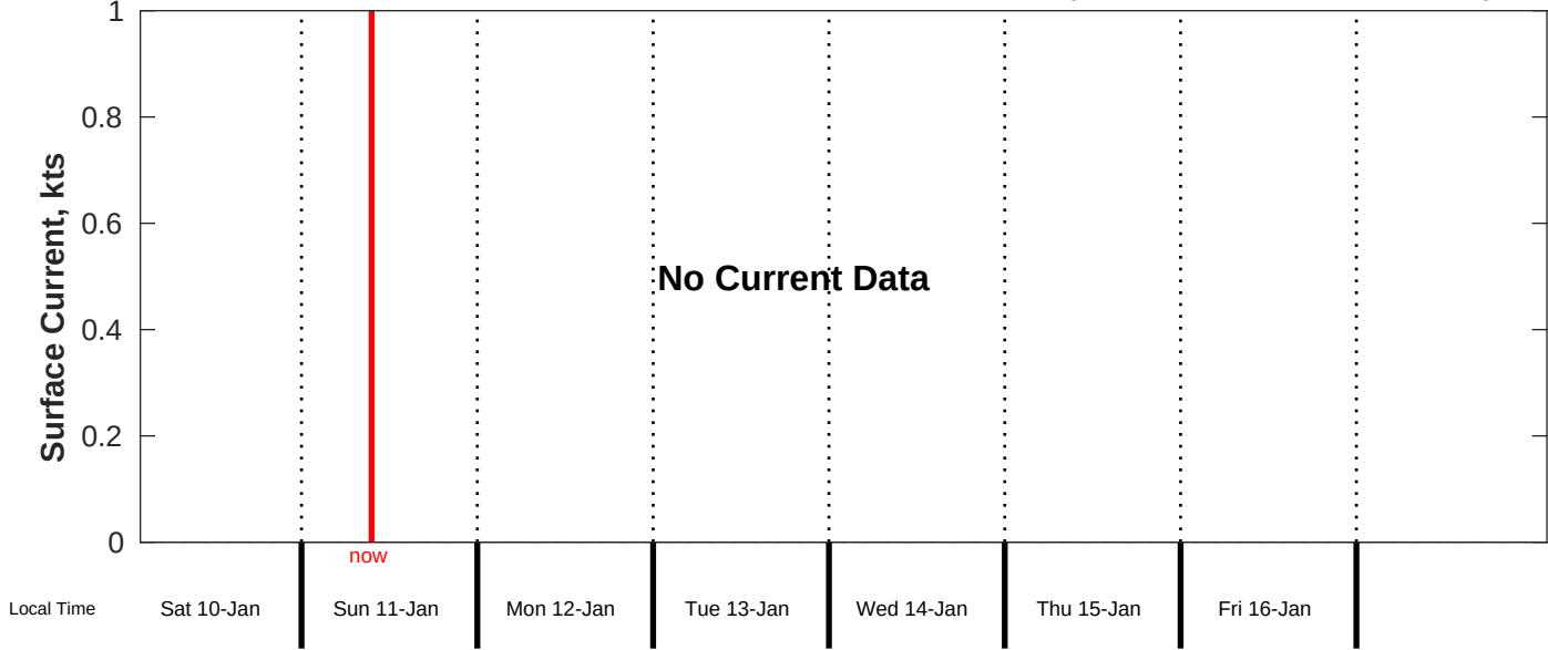
Surface Current Forecast for CSA (ONHYM) PPL EBS - Guinea from 10-Jan-2026 00:00:00 to 18-Jan-2026 00:00:00
