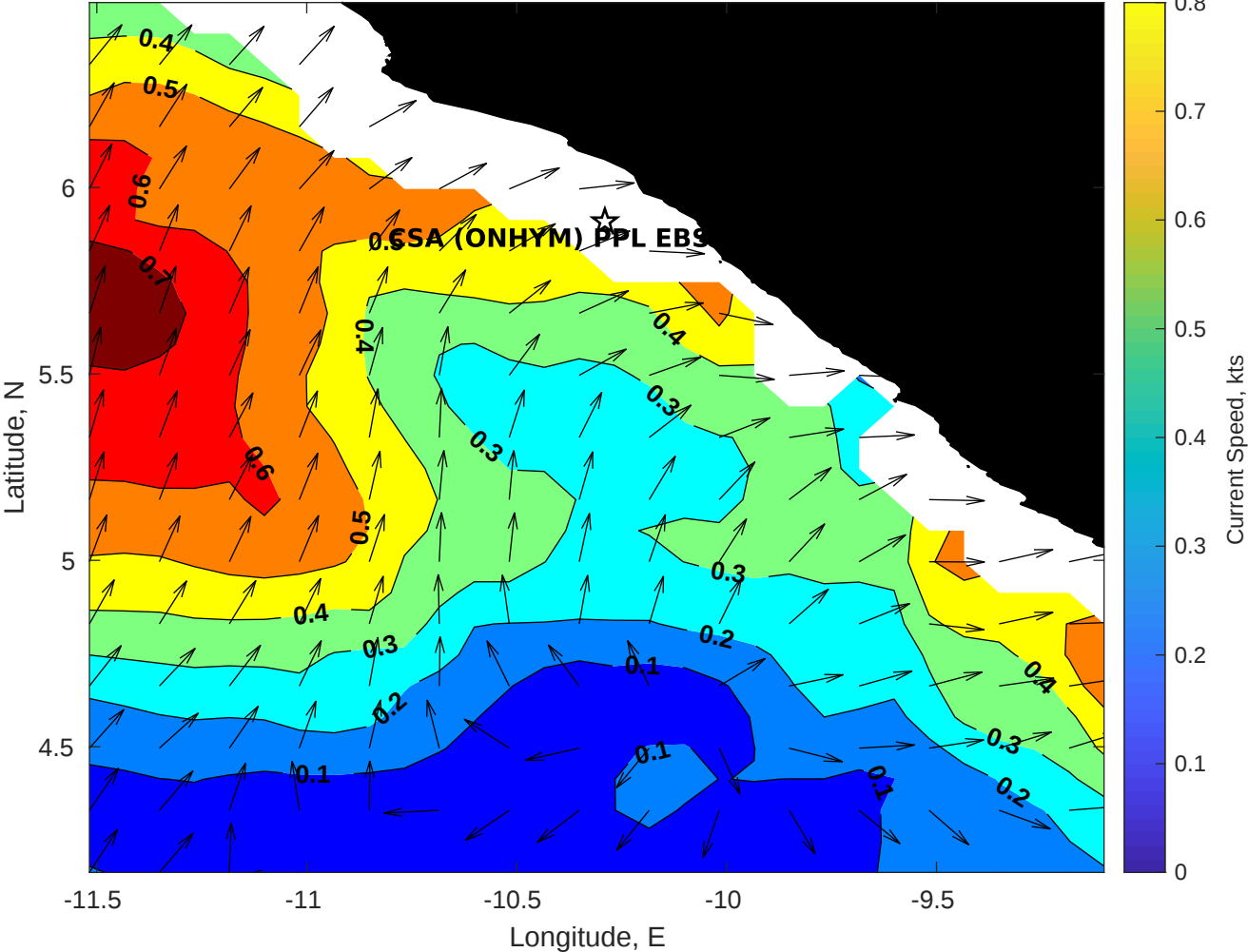
Surface Currents for CSA (ONHYM) PPL EBS - Liberia at 10-Jan-2026 00:00:00
