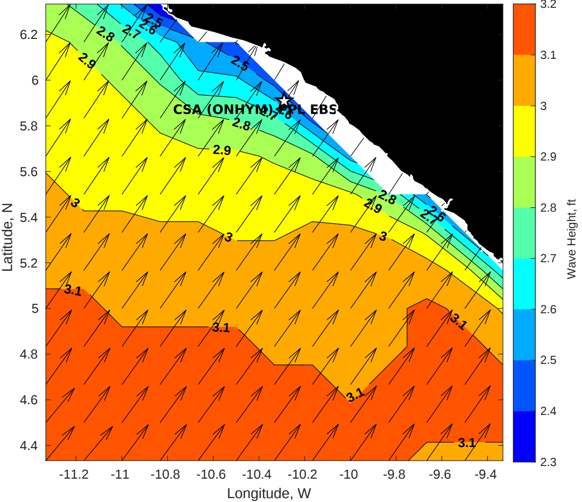
GFS Wave Height (ft) for CSA (ONHYM) PPL EBS - Liberia at 11-Jan-2026 09:00:00
