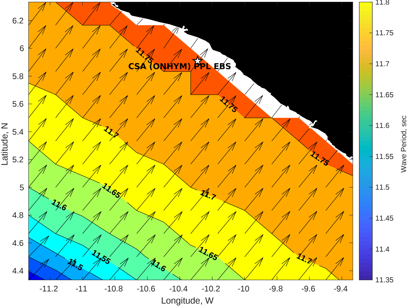
GFS Wave Period (sec) for CSA (ONHYM) PPL EBS - Liberia at 11-Jan-2026 09:00:00
