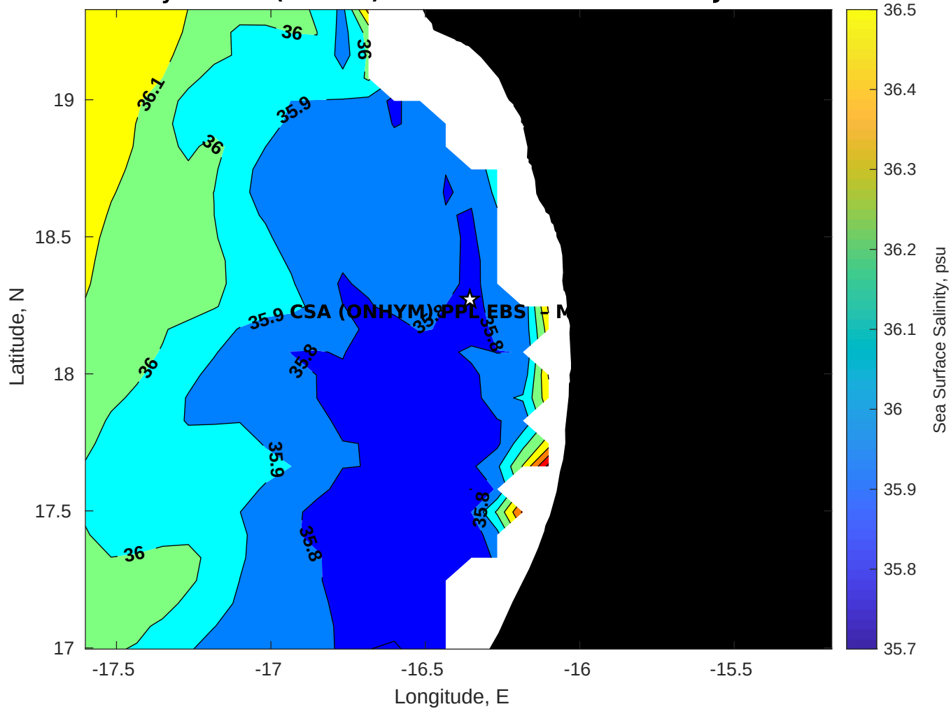
Surface Salinity for CSA (ONHYM) PPL EBS - Mauritania at 10-Jan-2026 00:00:00
