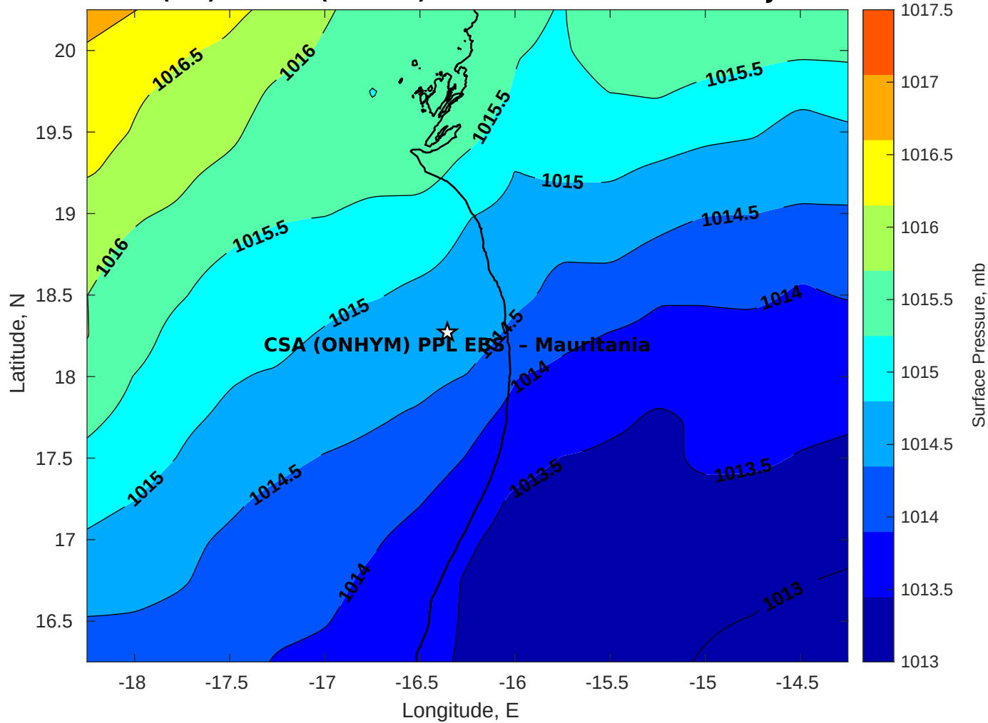
Surface Pressure (mb) for CSA (ONHYM) PPL EBS - Mauritania at 13-Jan-2026 00:00:00
