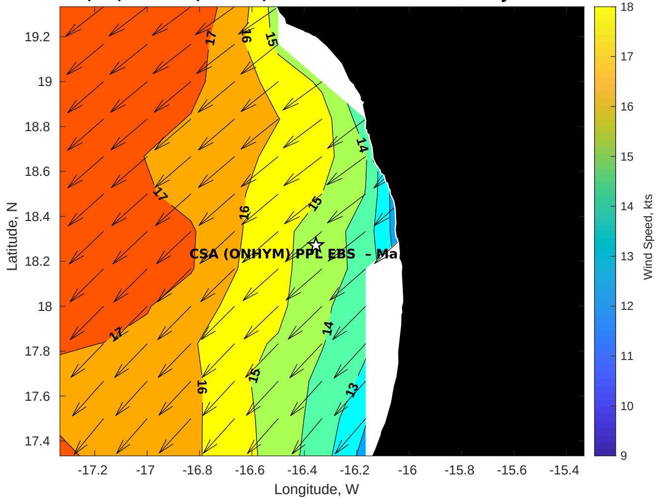
GFS Winds (kts) for CSA (ONHYM) PPL EBS - Mauritania at 11-Jan-2026 09:00:00
