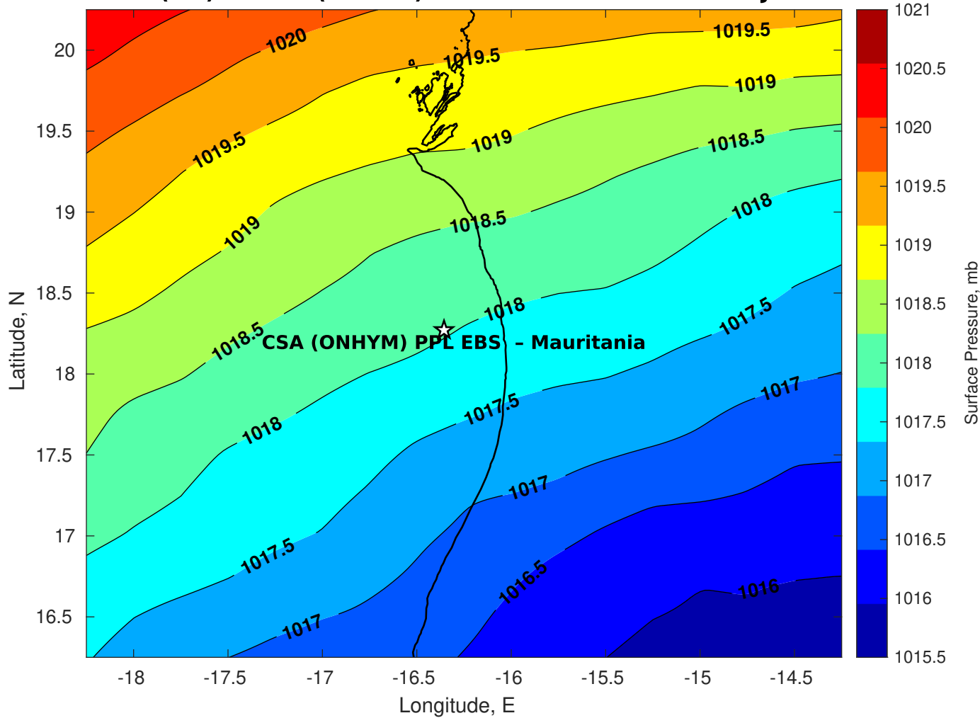
Surface Pressure (mb) for CSA (ONHYM) PPL EBS - Mauritania at 11-Jan-2026 00:00:00
