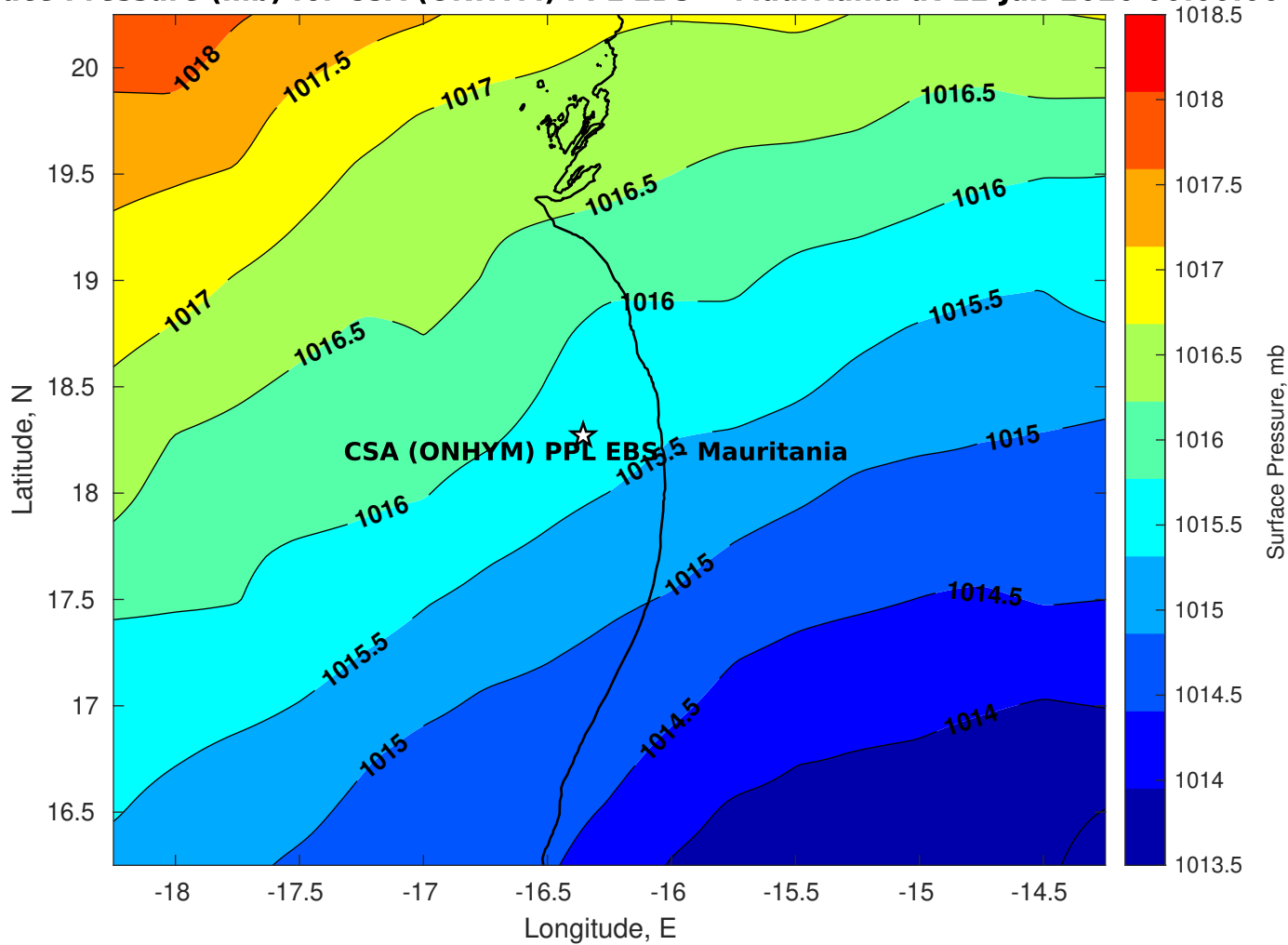
Surface Pressure (mb) for CSA (ONHYM) PPL EBS - Mauritania at 12-Jan-2026 00:00:00
