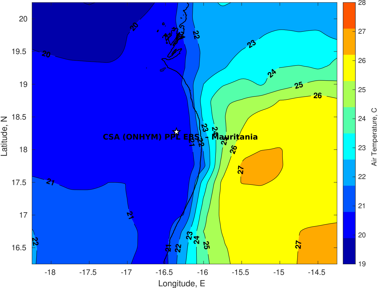
Air Temperature (C) for CSA (ONHYM) PPL EBS - Mauritania at 11-Jan-2026
