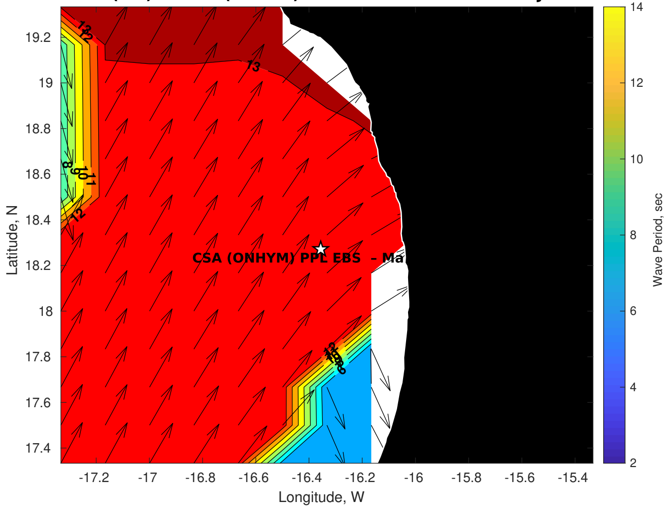
GFS Wave Period (sec) for CSA (ONHYM) PPL EBS - Mauritania at 11-Jan-2026 09:00:00
