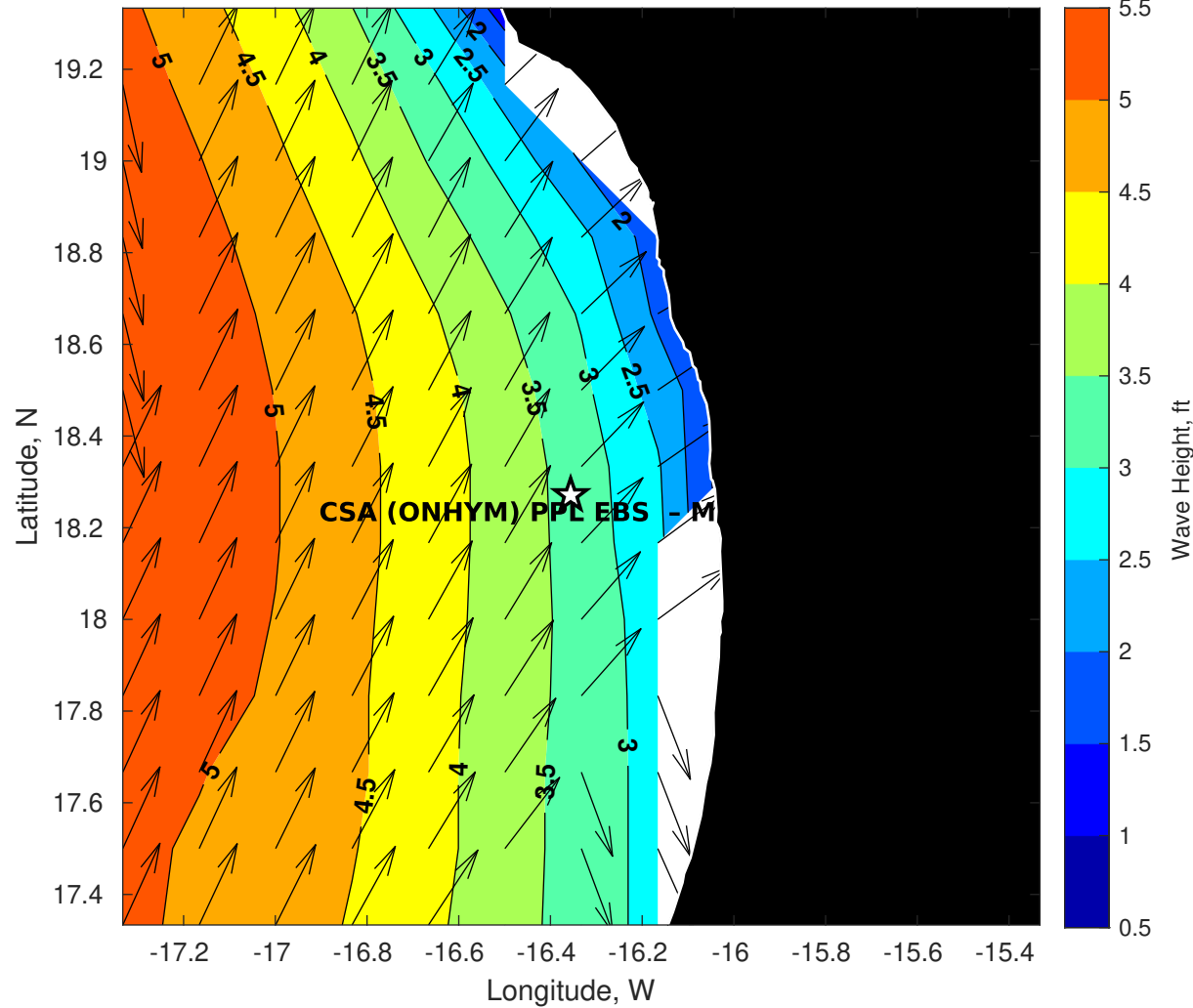
GFS Wave Height (ft) for CSA (ONHYM) PPL EBS - Mauritania at 11-Jan-2026 09:00:00
