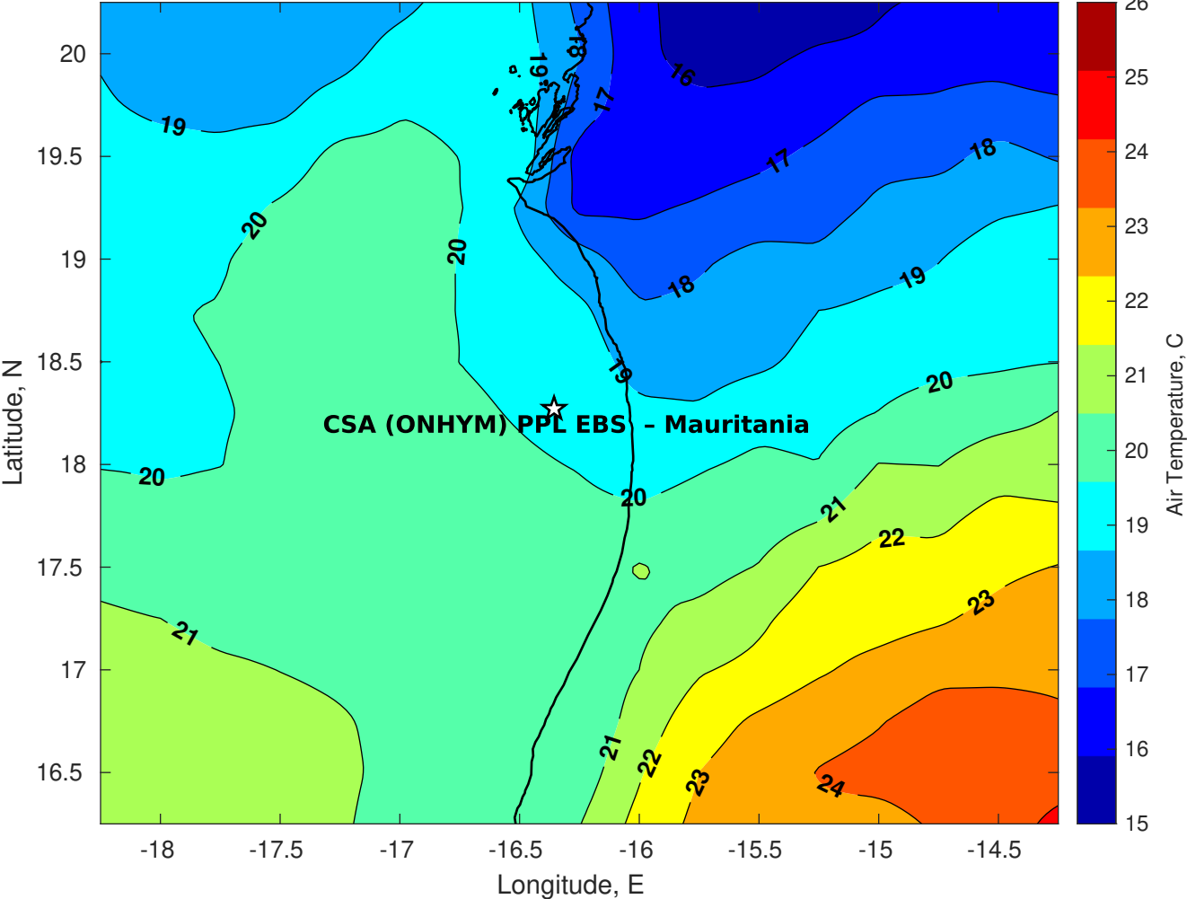
Air Temperature (C) for CSA (ONHYM) PPL EBS - Mauritania at 11-Jan-2026
