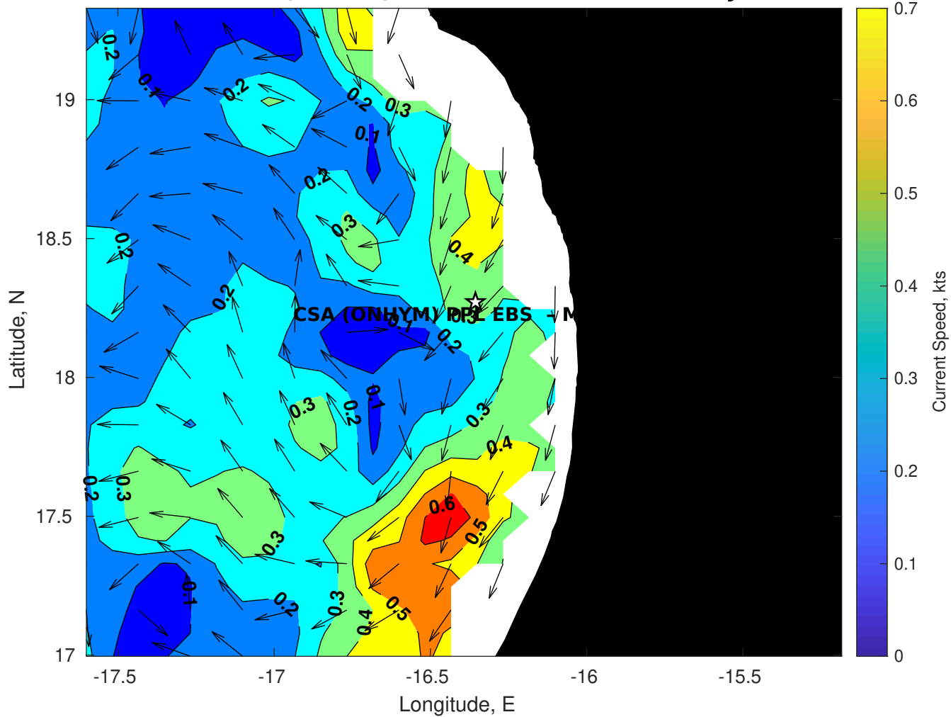
Surface Currents for CSA (ONHYM) PPL EBS - Mauritania at 10-Jan-2026 00:00:00
