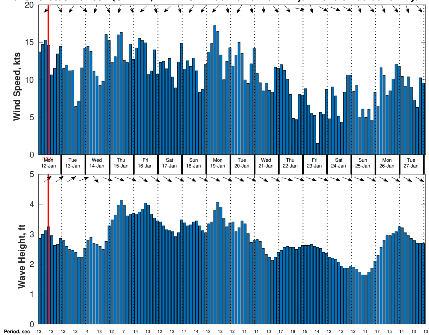
Wind & Wave Forecast for CSA (ONHYM) PPL EBS - Mauritania from 11-Jan-2026 01:00:00 to 27-Jan-2026 01:00:00
