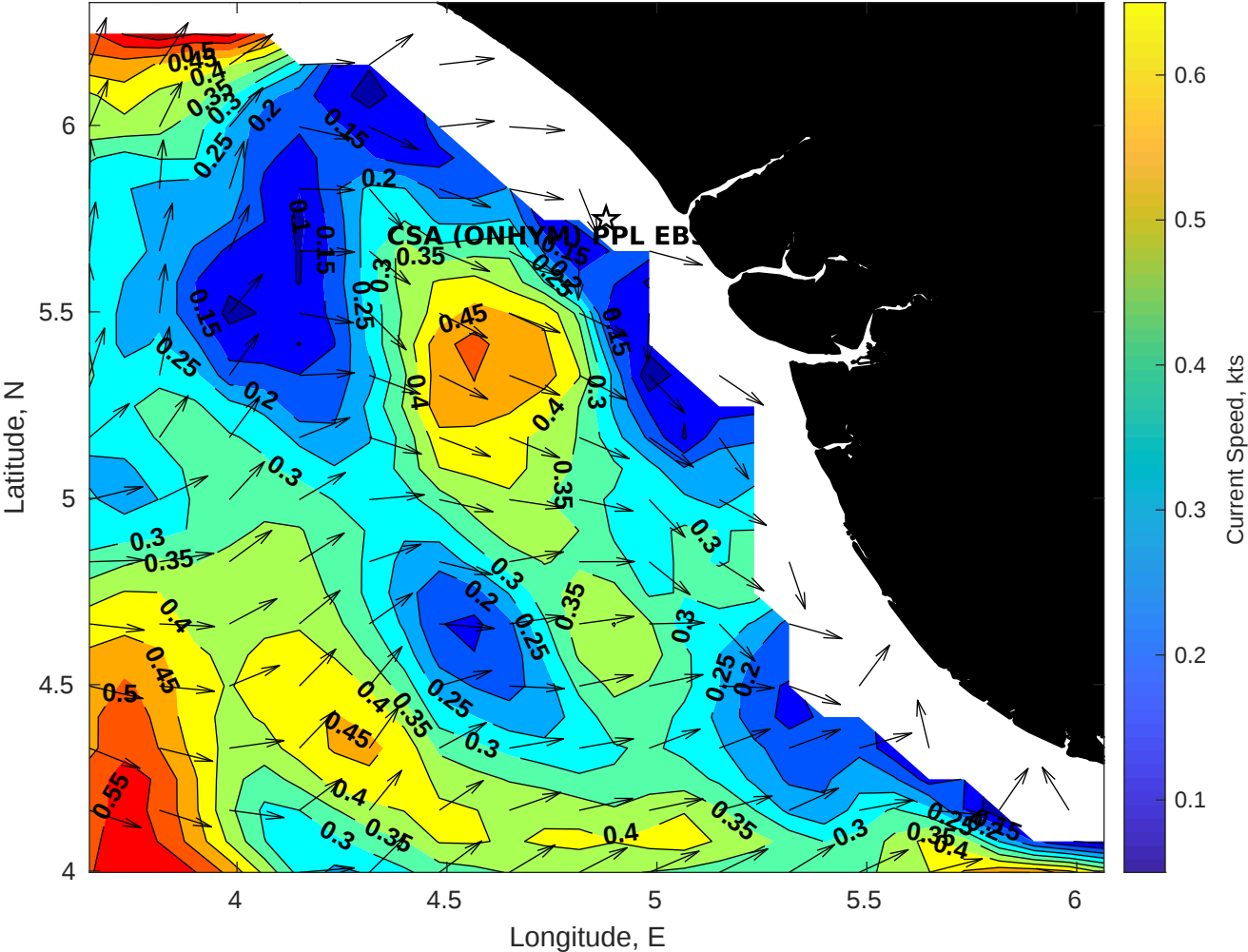
Surface Currents for CSA (ONHYM) PPL EBS - Nigeria at 10-Jan-2026 00:00:00
