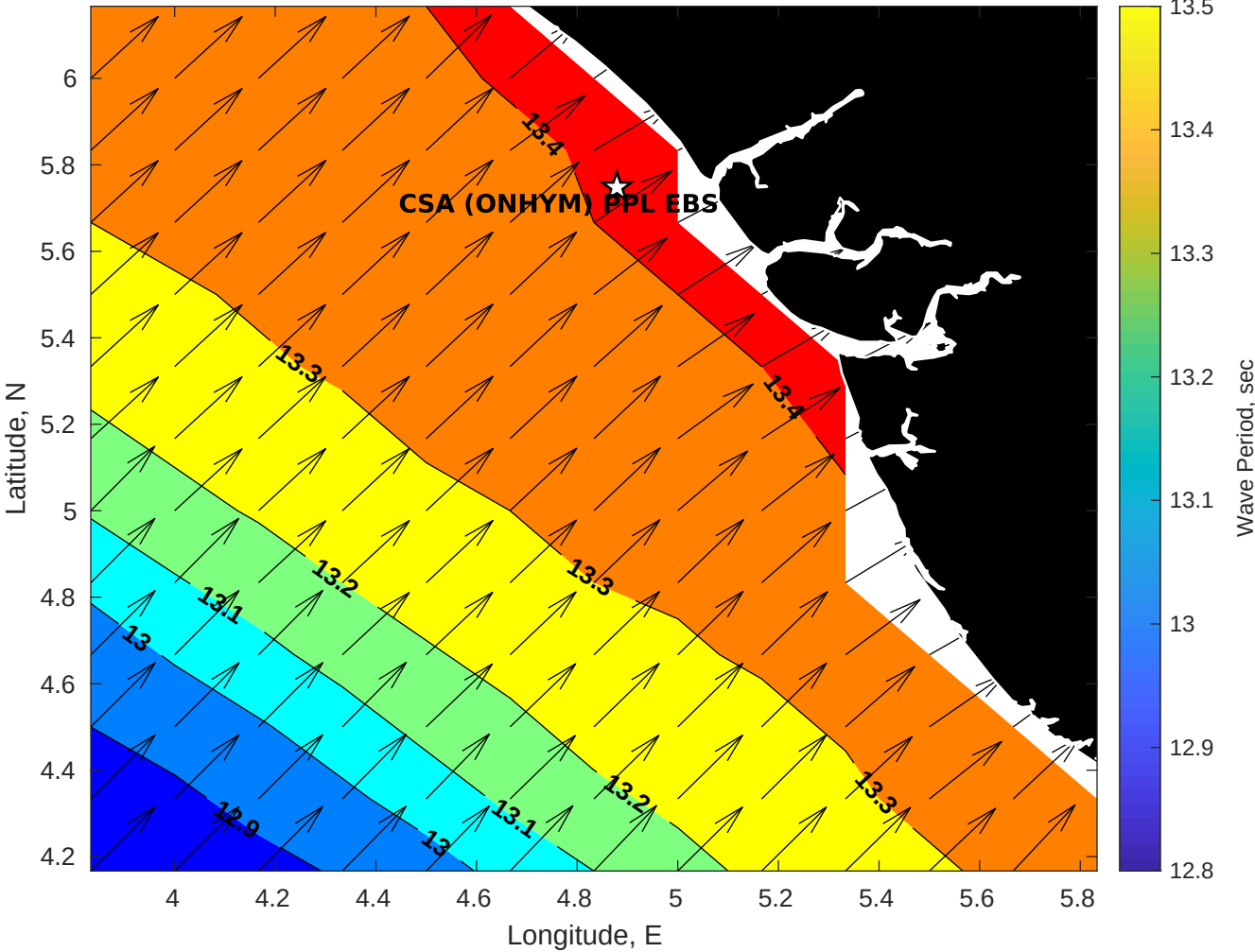
GFS Wave Period (sec) for CSA (ONHYM) PPL EBS - Nigeria at 11-Jan-2026 09:00:00
