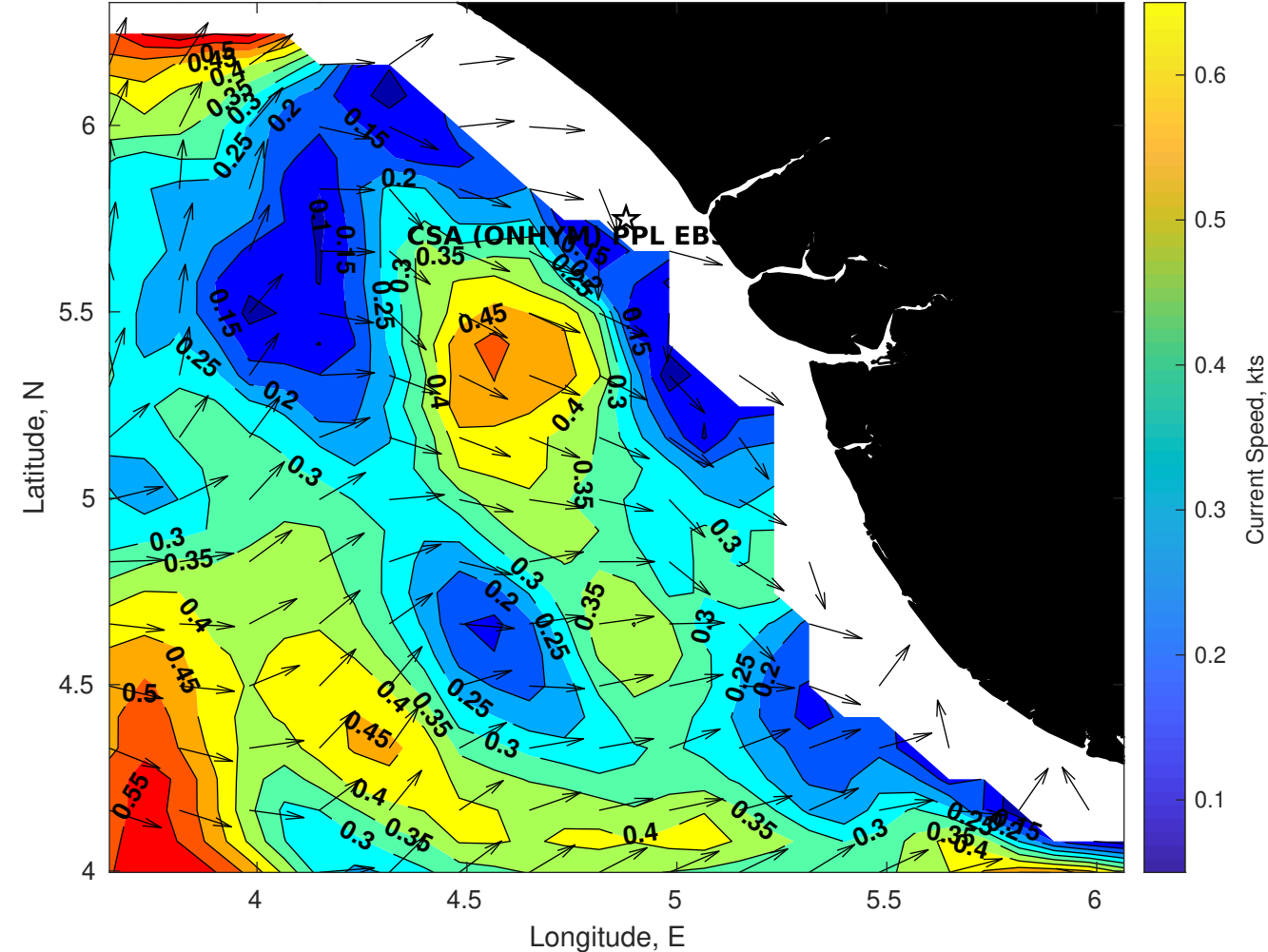
Surface Currents for CSA (ONHYM) PPL EBS - Nigeria at 10-Jan-2026 00:00:00
