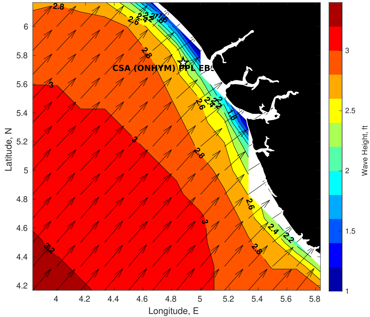
GFS Wave Height (ft) for CSA (ONHYM) PPL EBS - Nigeria at 11-Jan-2026 09:00:00
