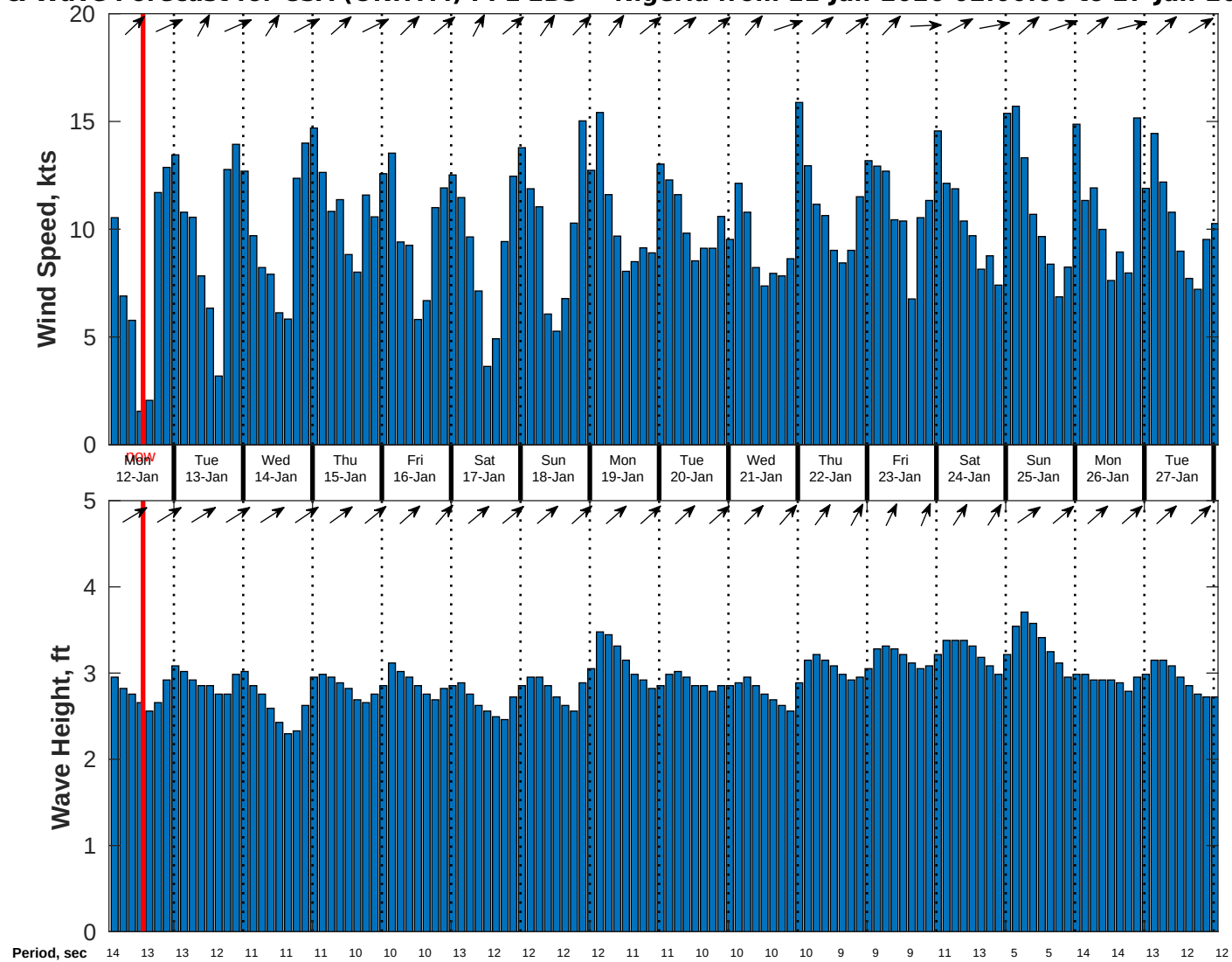
Wind & Wave Forecast for CSA (ONHYM) PPL EBS - Nigeria from 11-Jan-2026 02:00:00 to 27-Jan-2026 02:00:00
