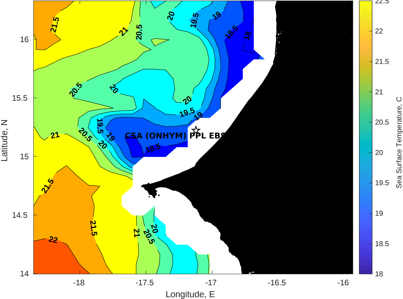
SST for CSA (ONHYM) PPL EBS - Senegal at 10-Jan-2026 00:00:00
