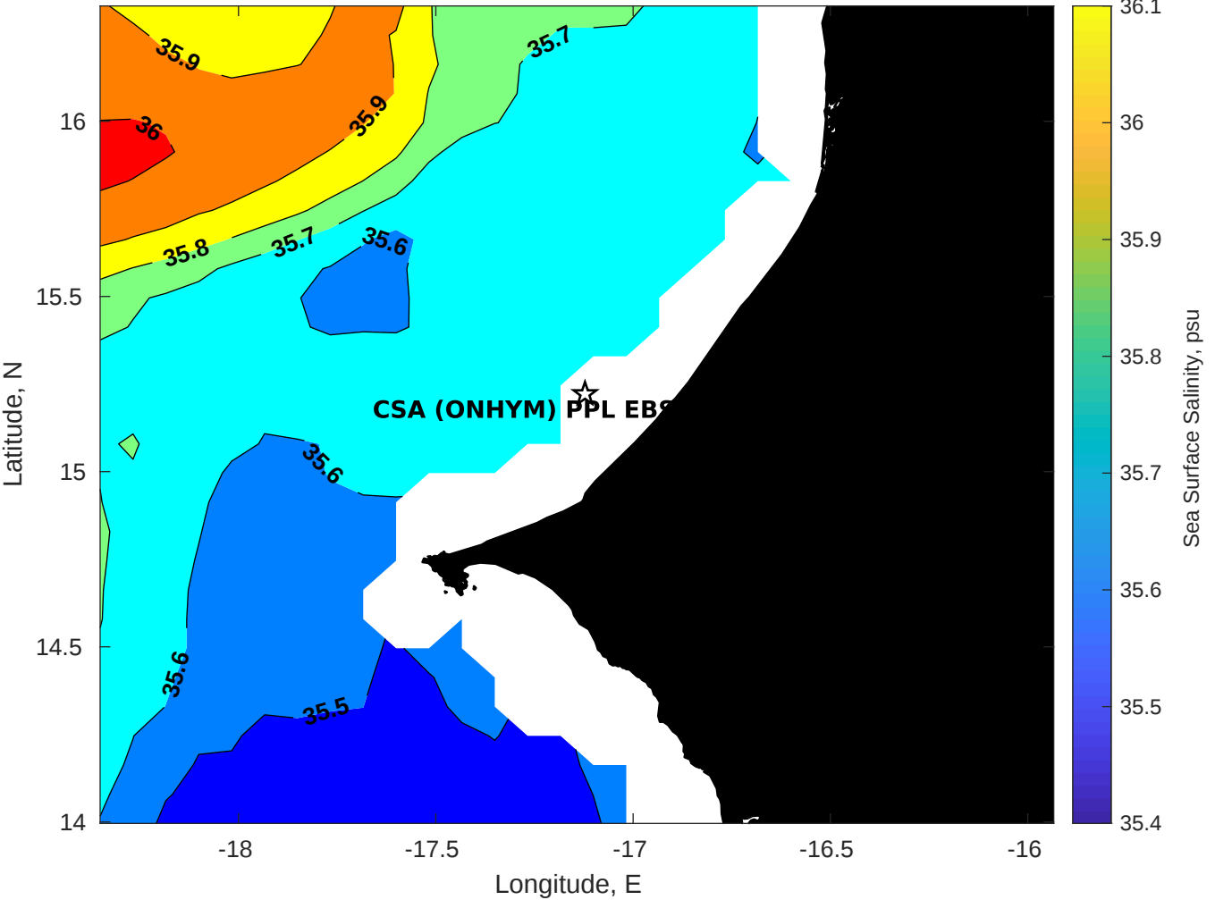
Surface Salinity for CSA (ONHYM) PPL EBS - Senegal at 10-Jan-2026 00:00:00
