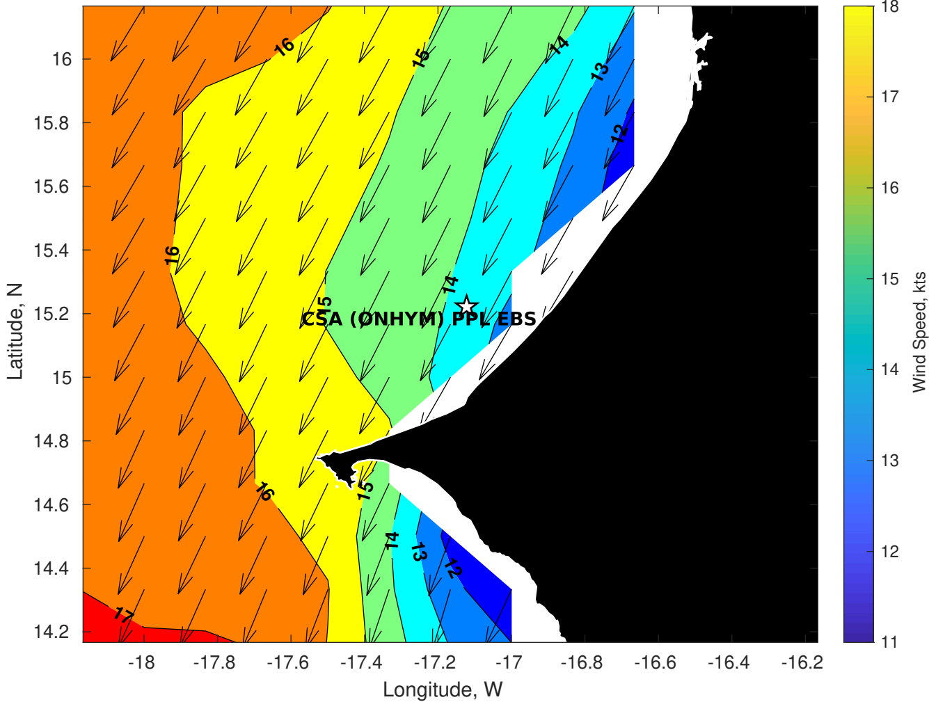
GFS Winds (kts) for CSA (ONHYM) PPL EBS - Senegal at 11-Jan-2026 09:00:00
