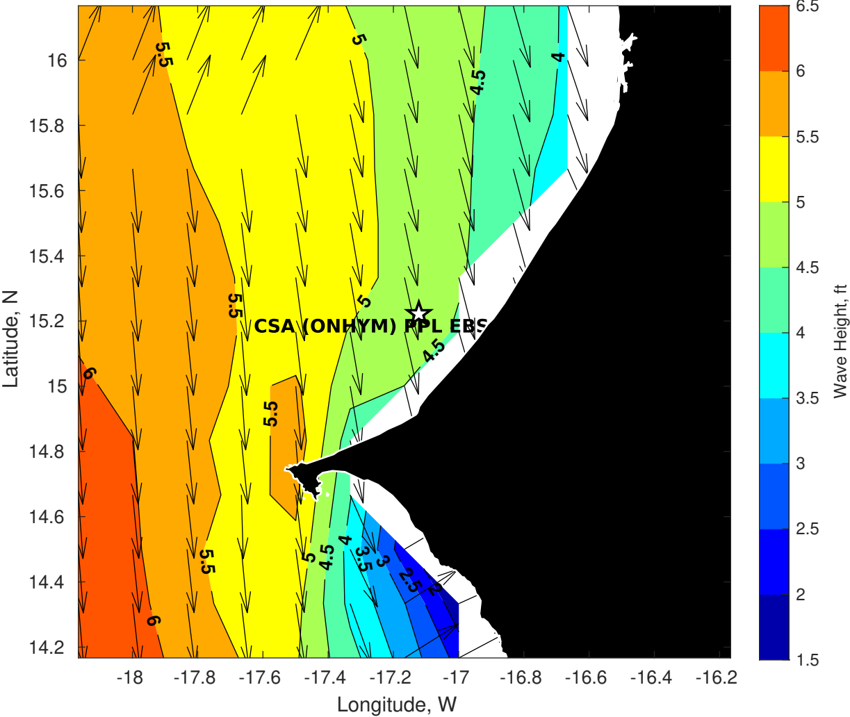
GFS Wave Height (ft) for CSA (ONHYM) PPL EBS - Senegal at 11-Jan-2026 09:00:00
