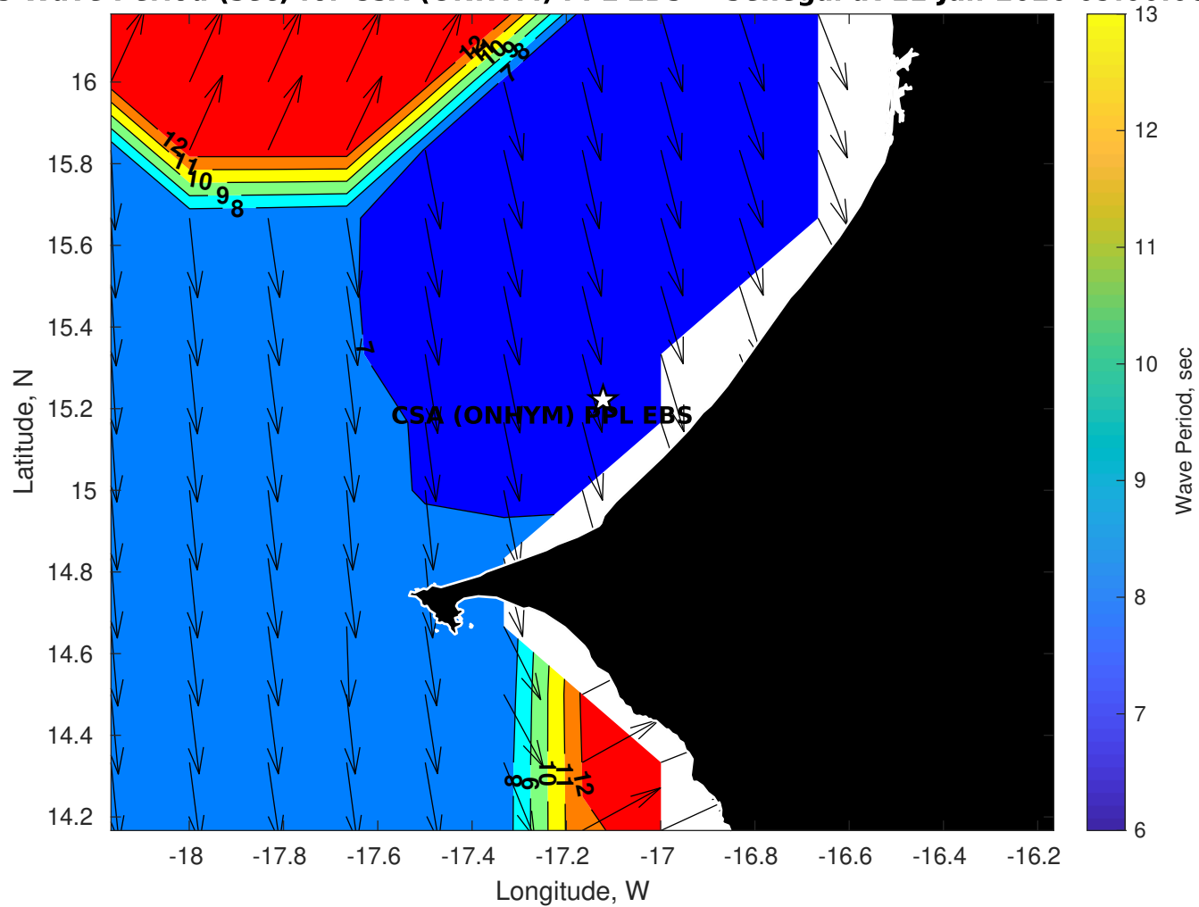
GFS Wave Period (sec) for CSA (ONHYM) PPL EBS - Senegal at 11-Jan-2026 09:00:00
