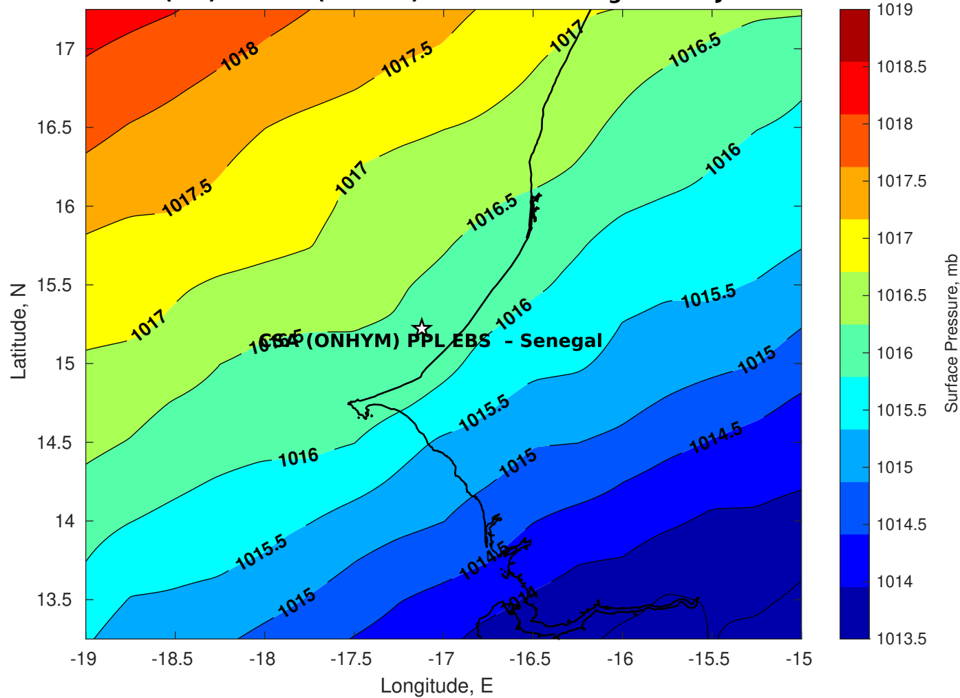
Surface Pressure (mb) for CSA (ONHYM) PPL EBS - Senegal at 11-Jan-2026 00:00:00
