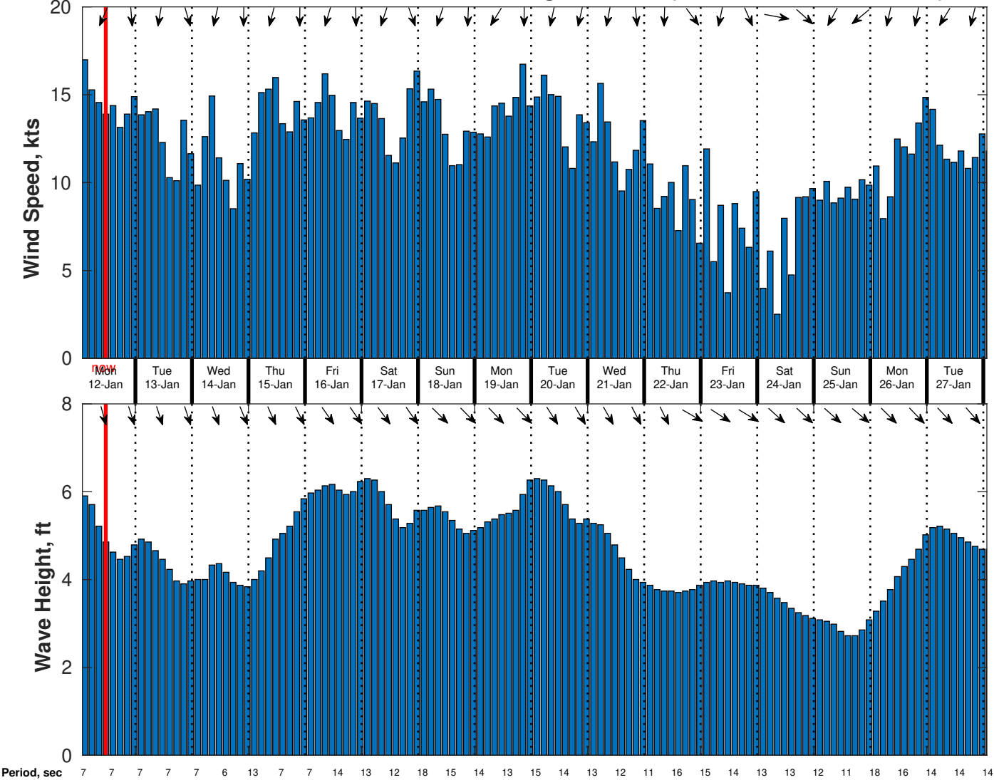
Wind & Wave Forecast for CSA (ONHYM) PPL EBS - Senegal from 11-Jan-2026 01:00:00 to 27-Jan-2026 01:00:00
