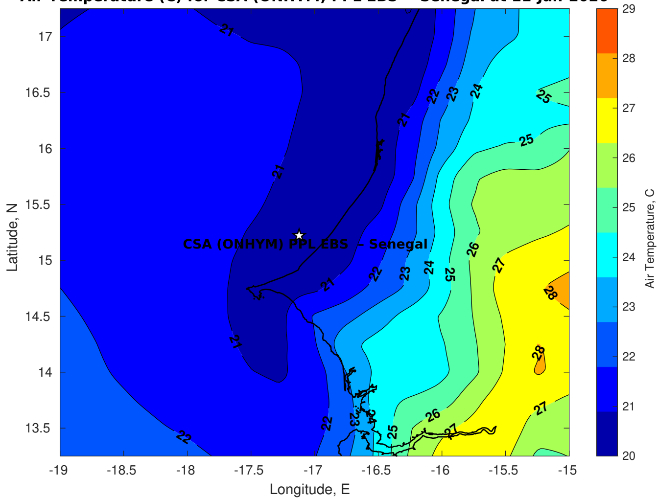
Air Temperature (C) for CSA (ONHYM) PPL EBS - Senegal at 11-Jan-2026
