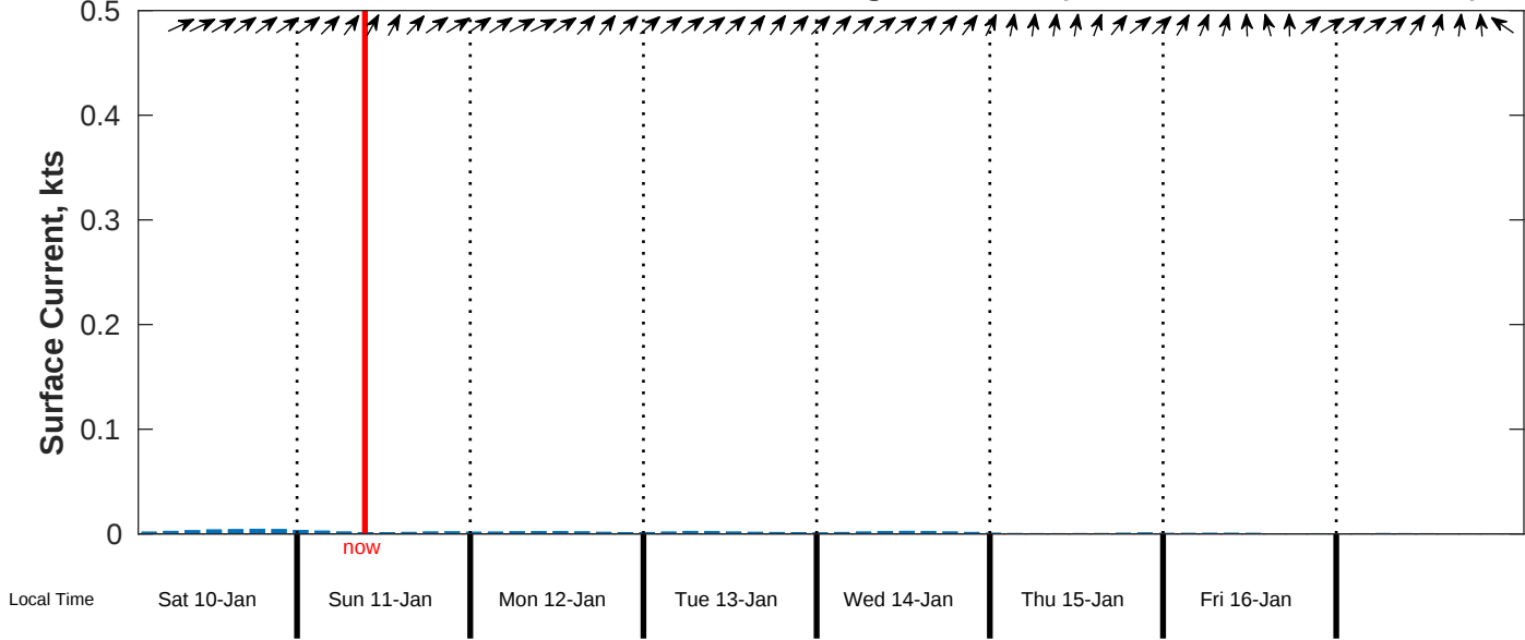
Surface Current Forecast for CSA (ONHYM) PPL EBS - Senegal from 10-Jan-2026 00:00:00 to 18-Jan-2026 00:00:00
