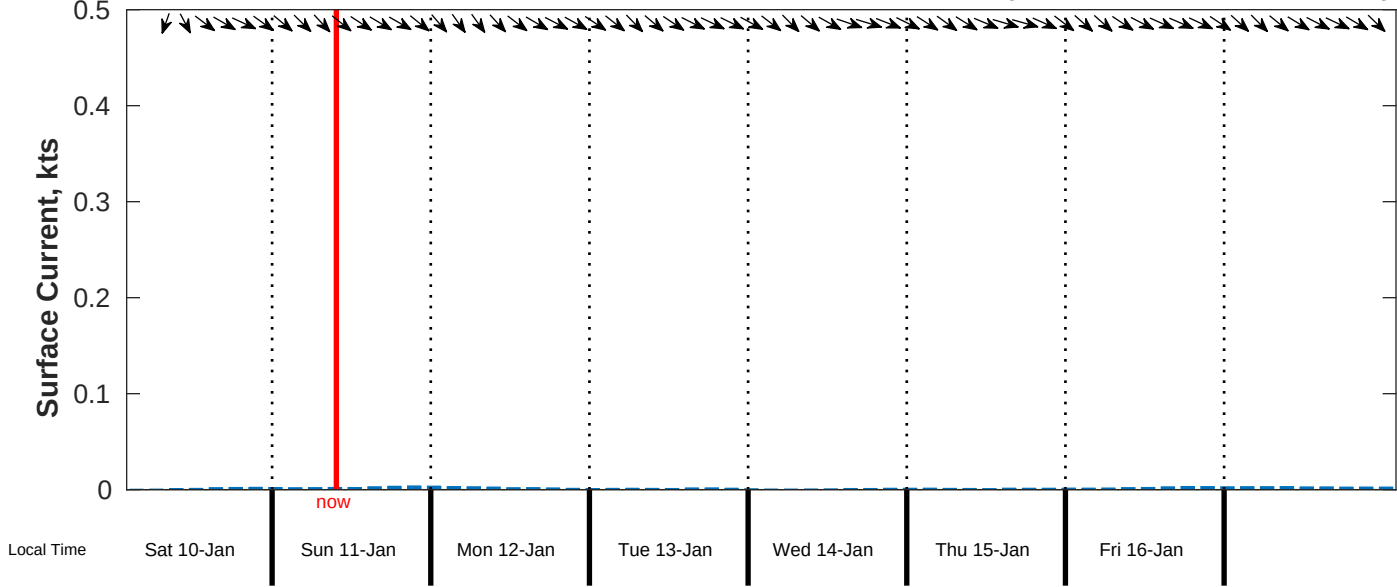
Surface Current Forecast for CSA (ONHYM) PPL EBS - Sierra Leone from 10-Jan-2026 00:00:00 to 18-Jan-2026 00:00:00
