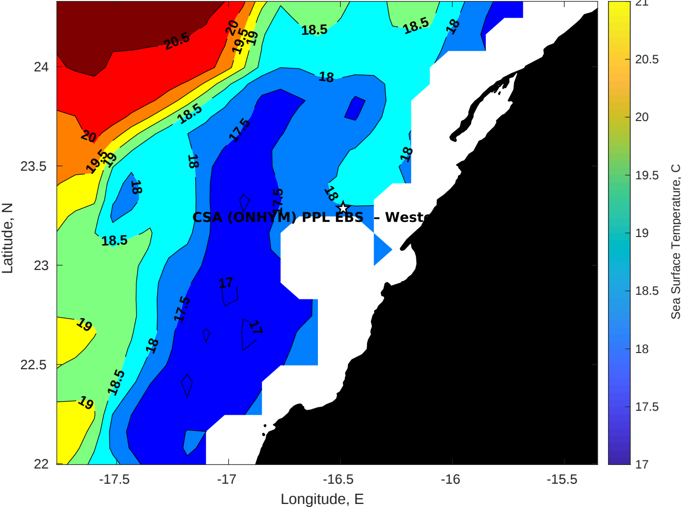
SST for CSA (ONHYM) PPL EBS - Western Sahara at 10-Jan-2026 00:00:00
